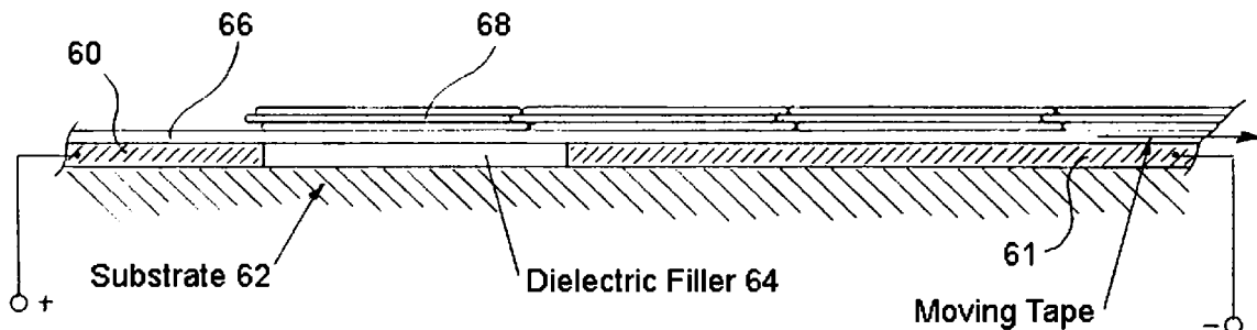
Formation of Nanotube Wires or Yarn
