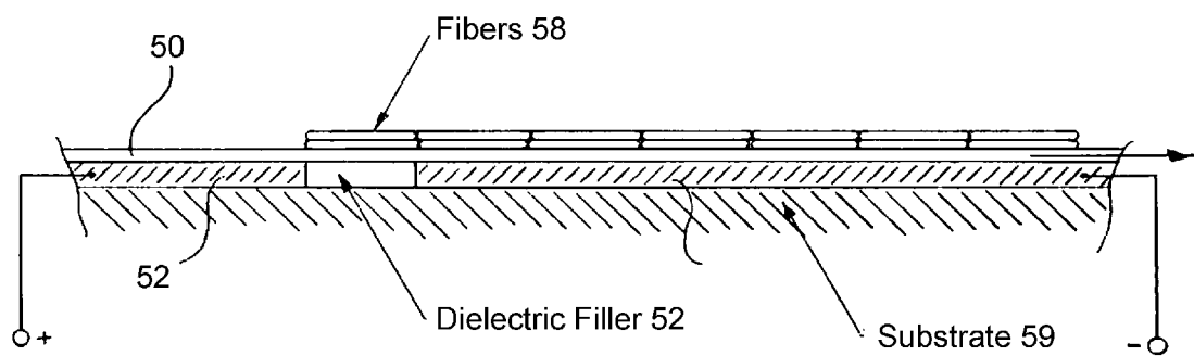
Dielectrophoretic Alignment of Fibers Across a Wide Web
