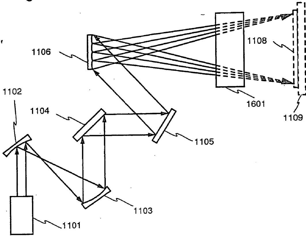
Fig. 6A top view
