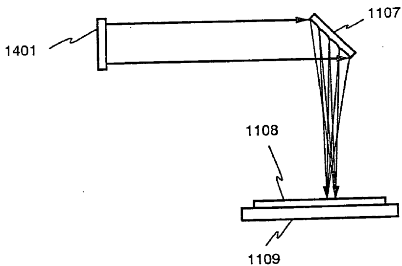
Fig. 4B side view
