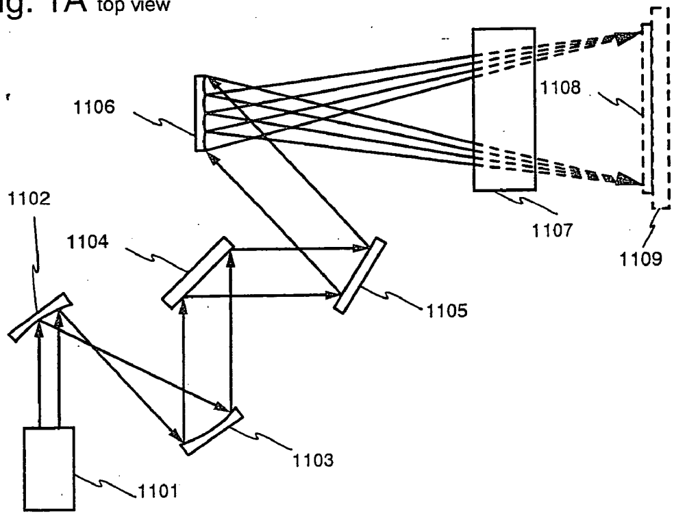
Fig. 1A top view
