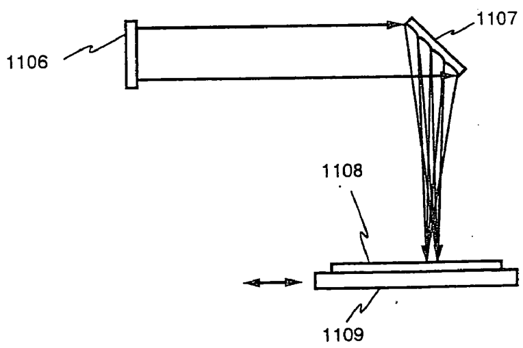
Fig. 1B side view
