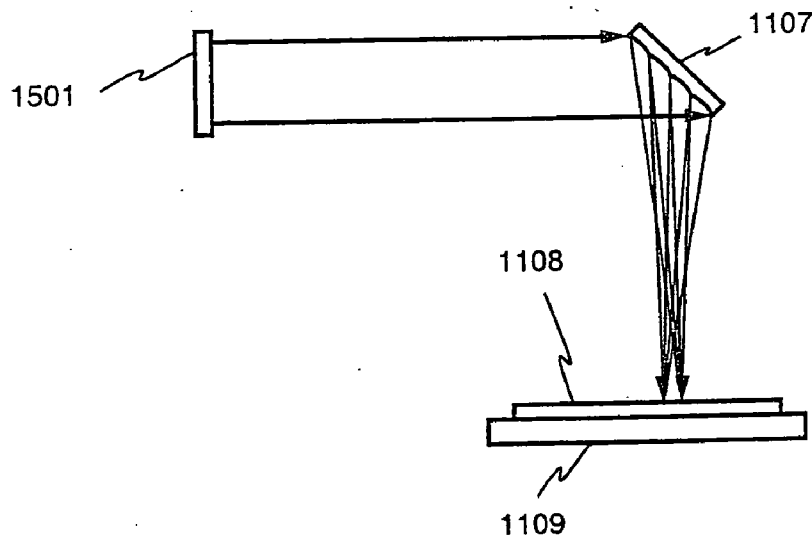
Fig. 5B side view
