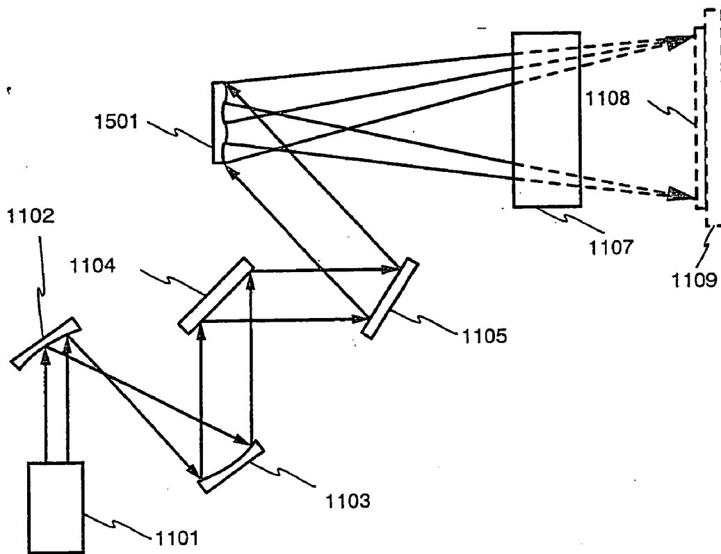
Fig. 5A top view
