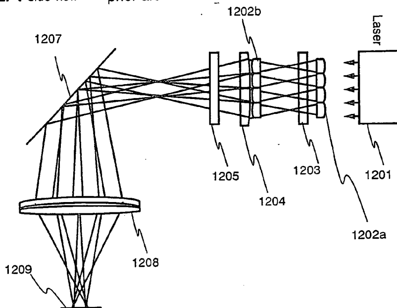
Fig. 2A side view prior art
