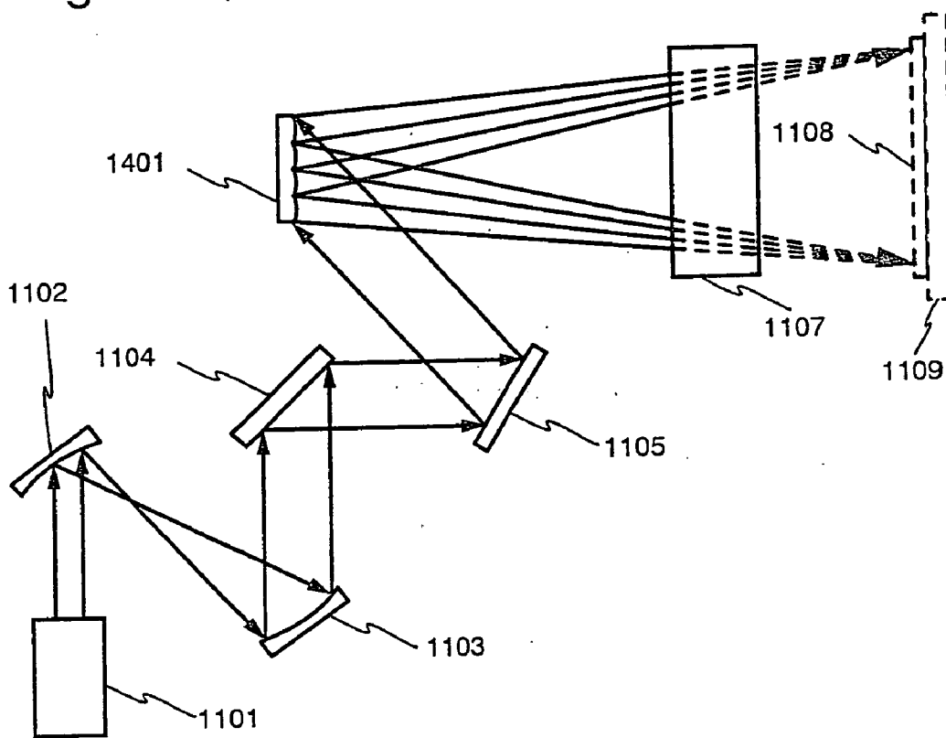
Fig. 4A top view
