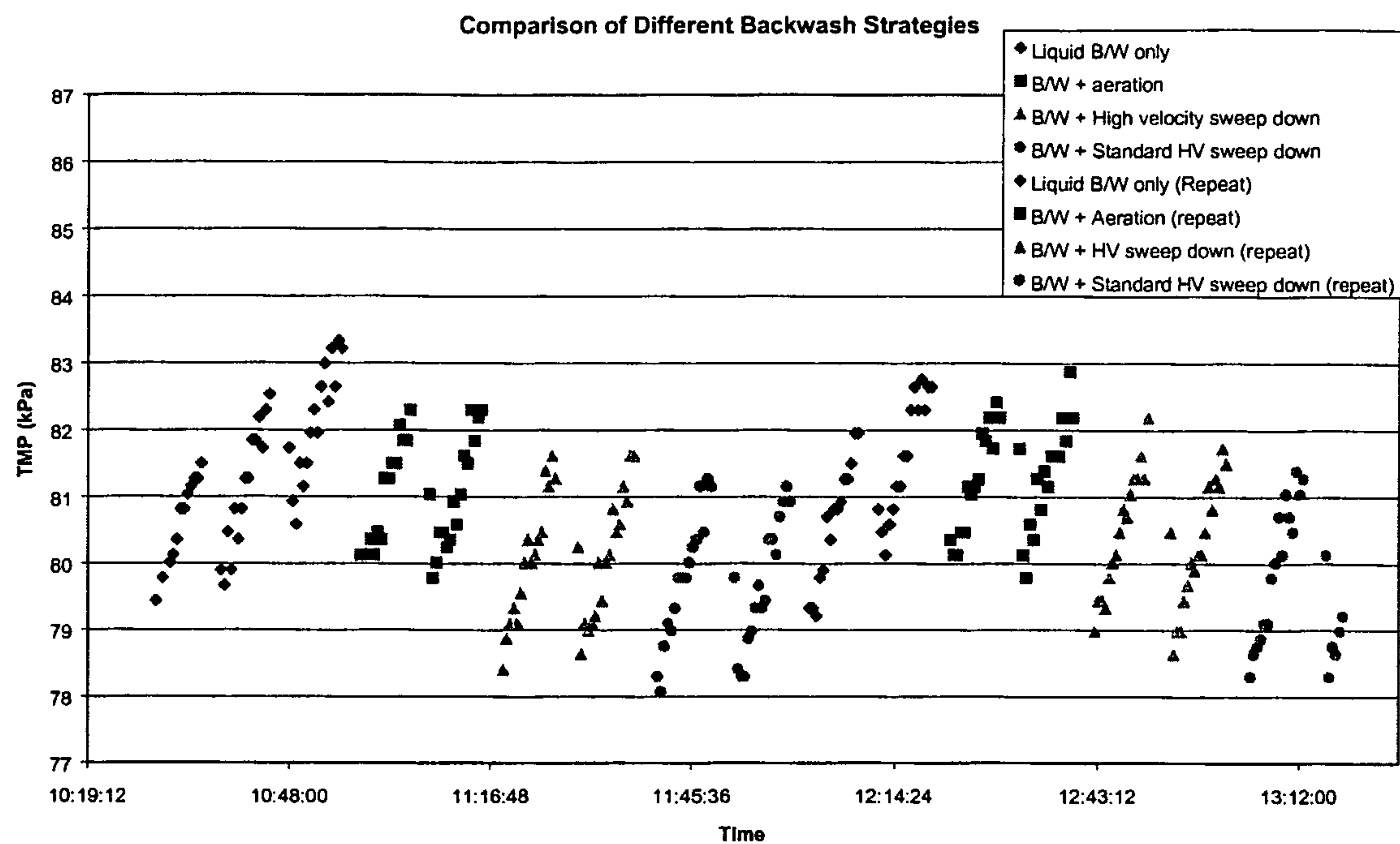
Figure 3 Cleaning Efficiency of Different Strategies
