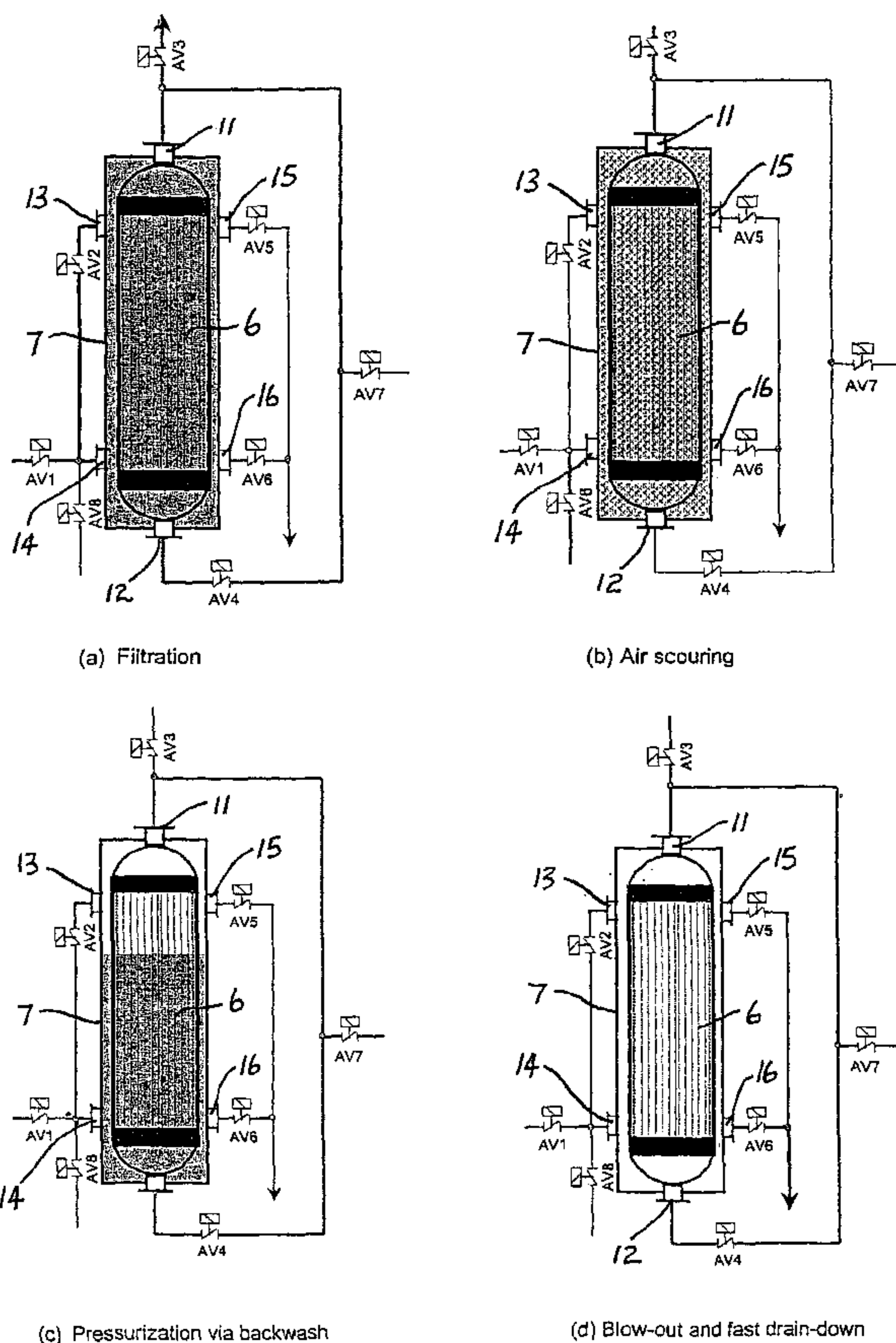
Membrane Cleaning Sequence
