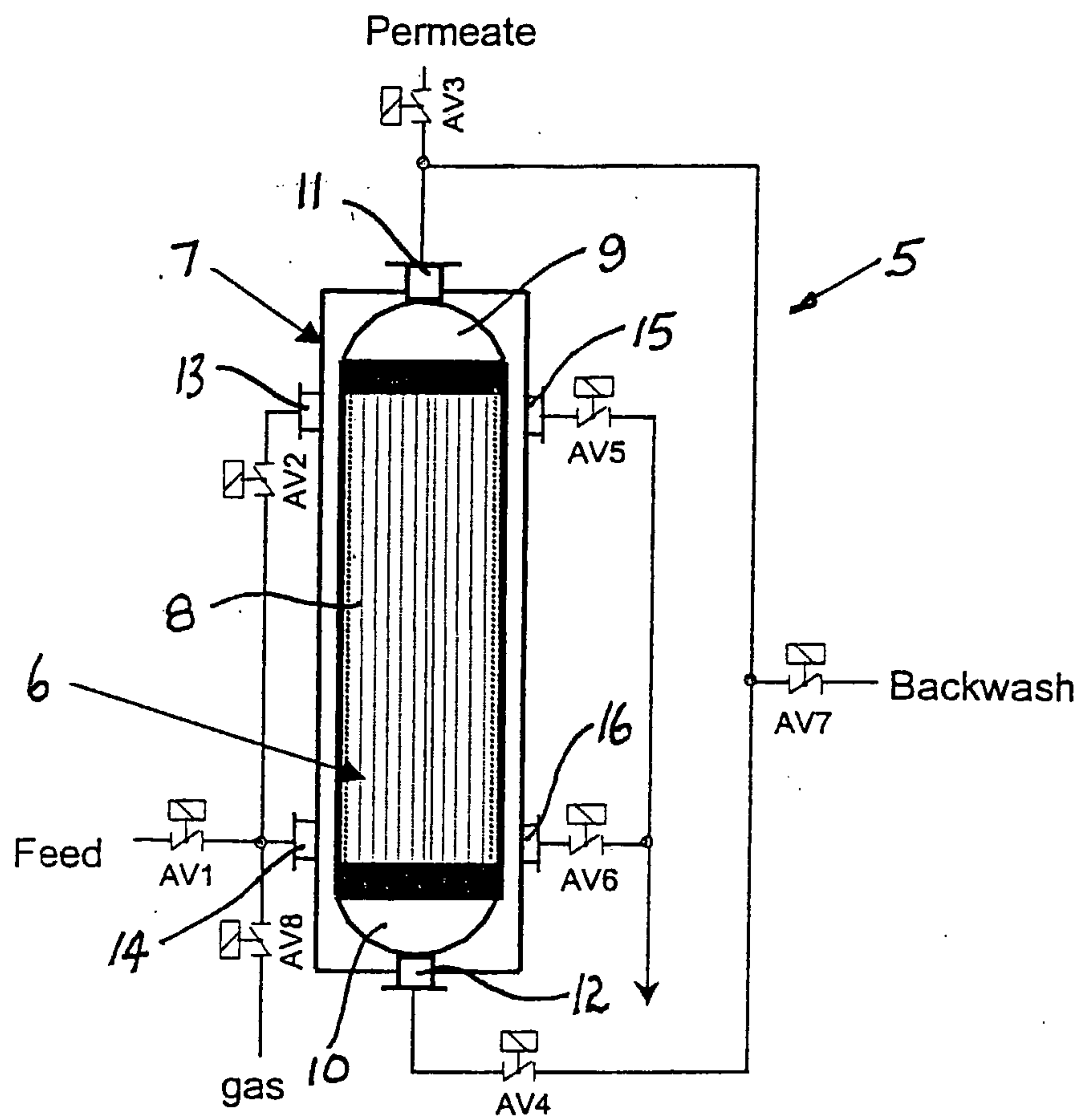
Figure 1 Membrane Module Assembly
