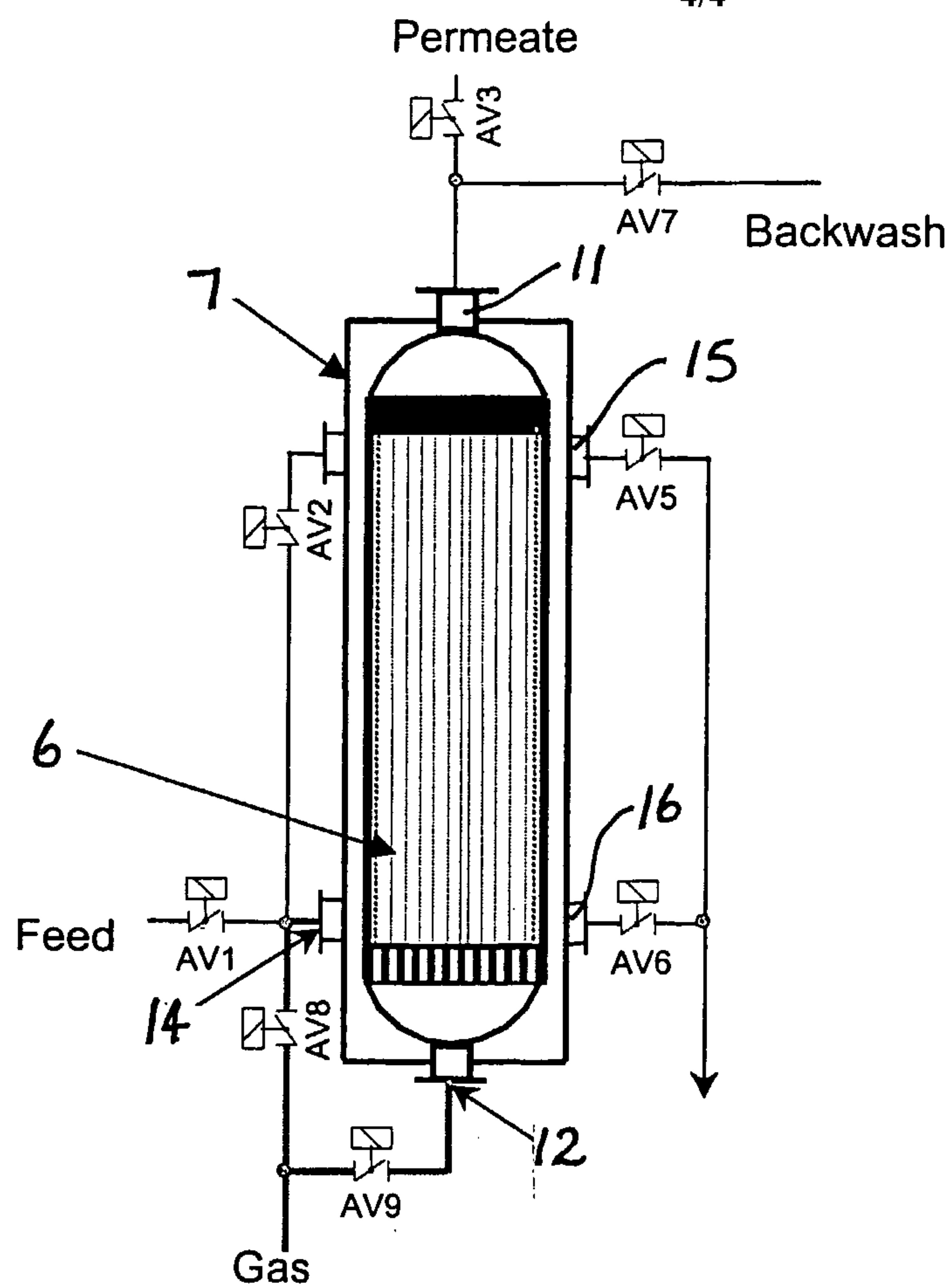
Figure 5 Alternative Air Injection
