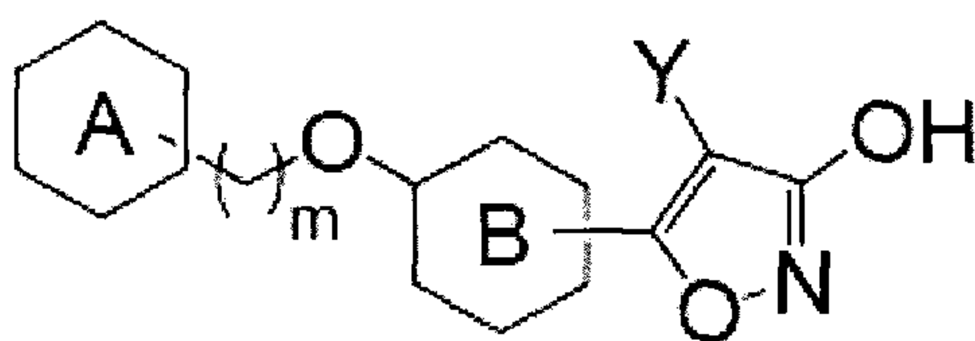
( I - 1 )
