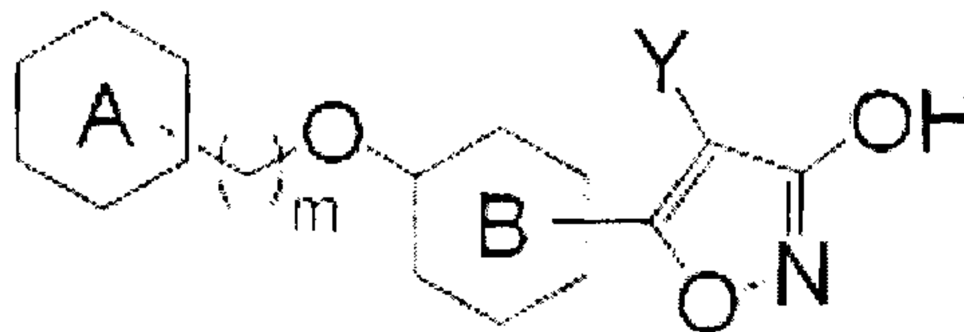
( I - 1 )
