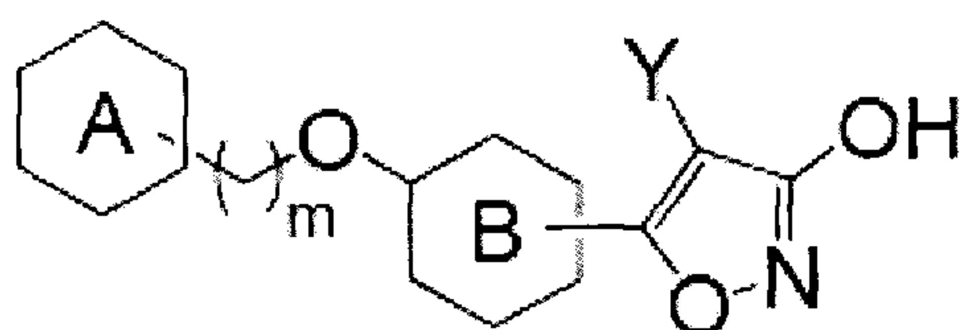
( I - 1 )
