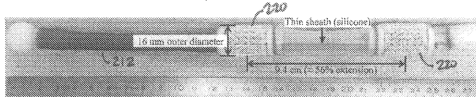
b). Device expanded with deflated attachments
