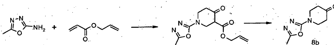
Scheme 23
