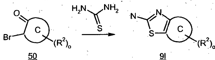
Scheme 16
