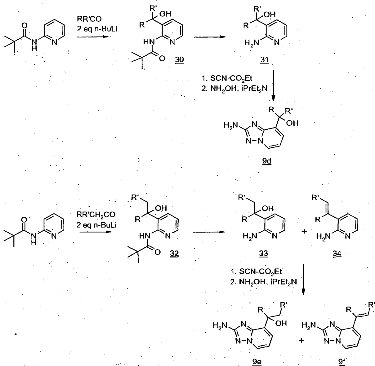
Scheme 11
