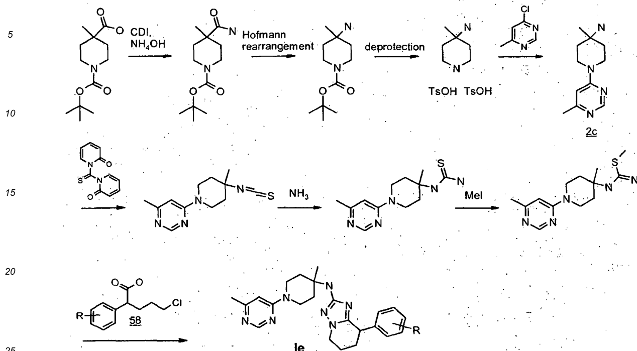
Scheme 32
