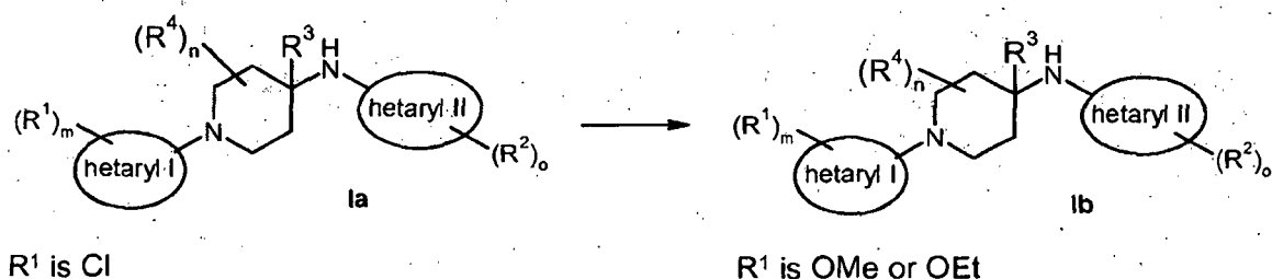
Scheme 29
