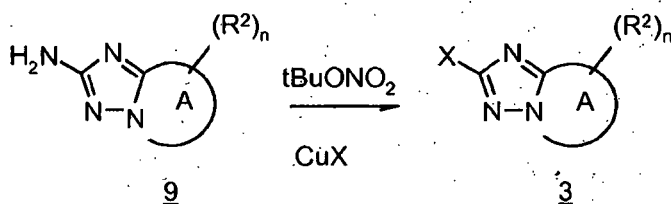
Scheme 17
