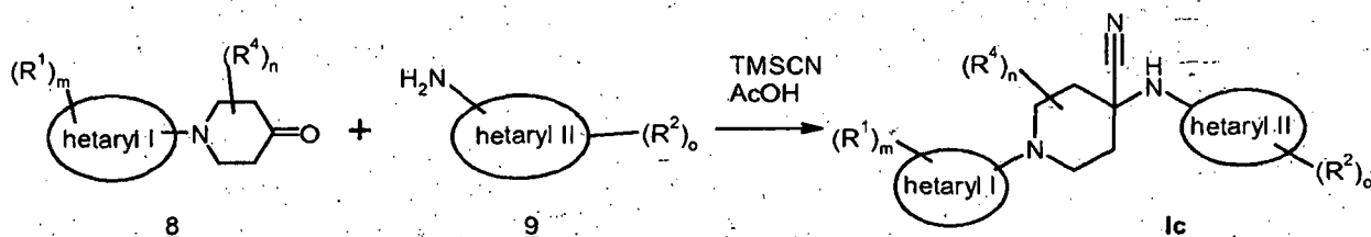
Scheme 30
