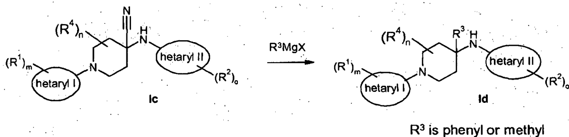
Scheme 31
