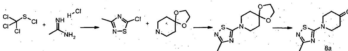
Scheme 22
