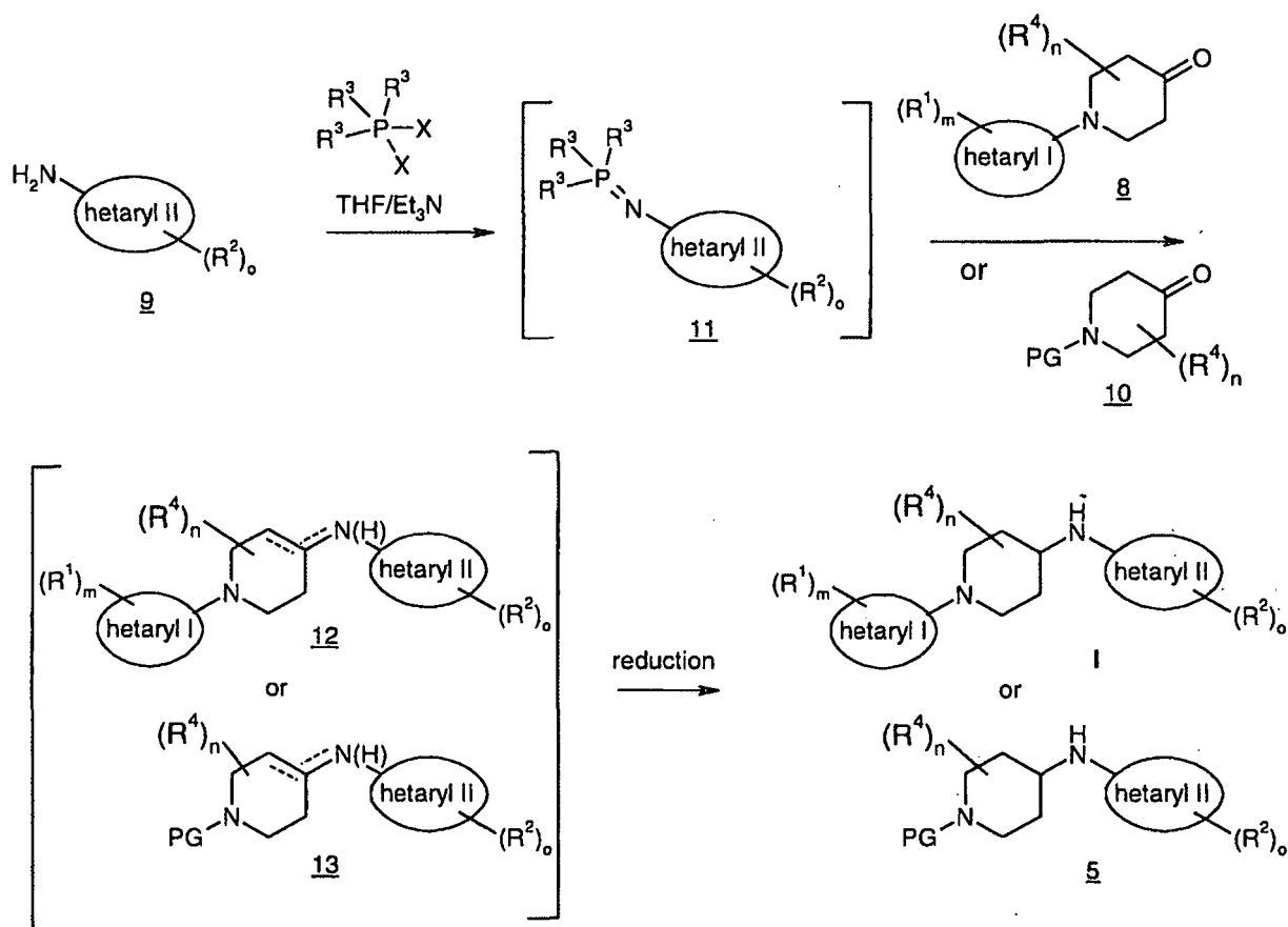
Scheme 4
