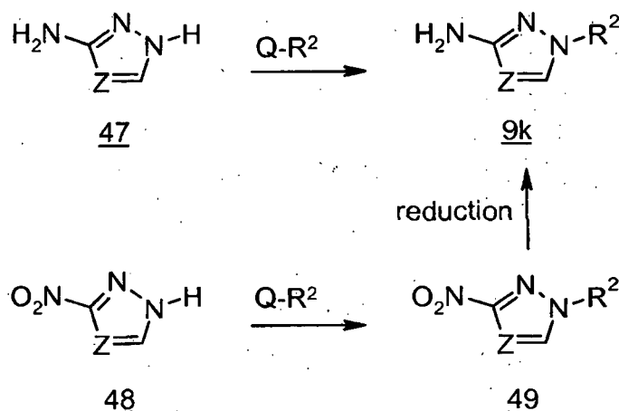
Scheme 15
