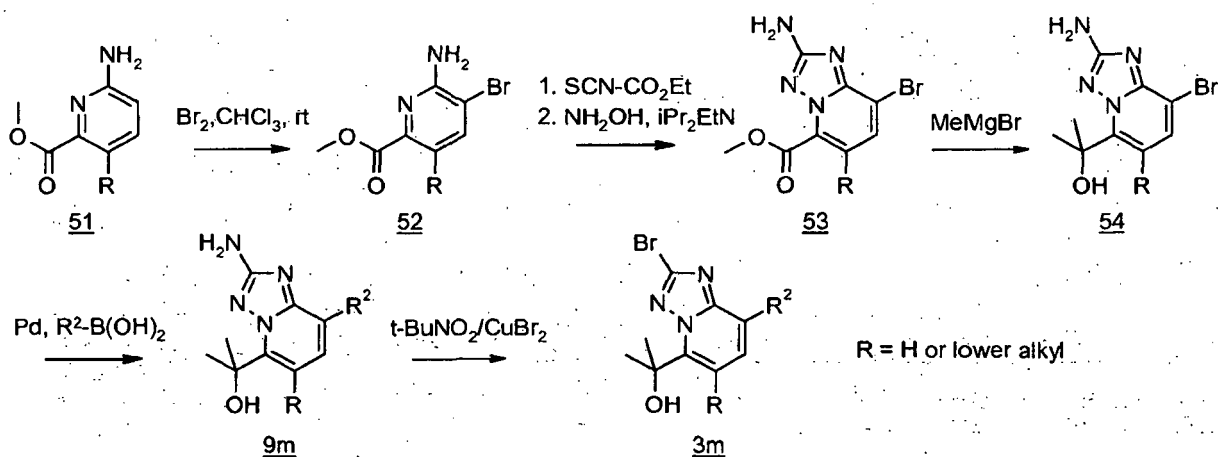
Scheme 18
