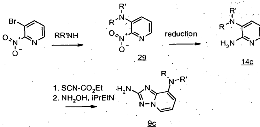
Scheme 10
