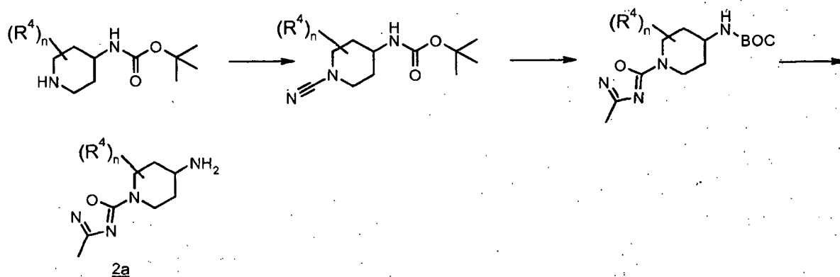
Scheme 25
