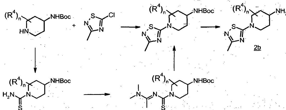
Scheme 26
