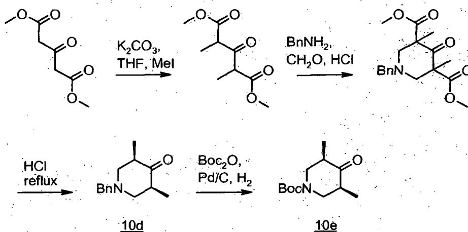
Scheme 21
