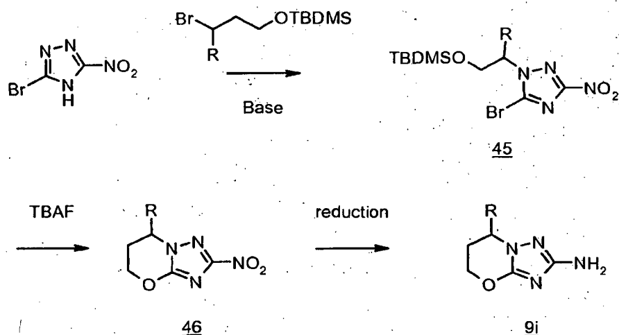
Scheme 14
