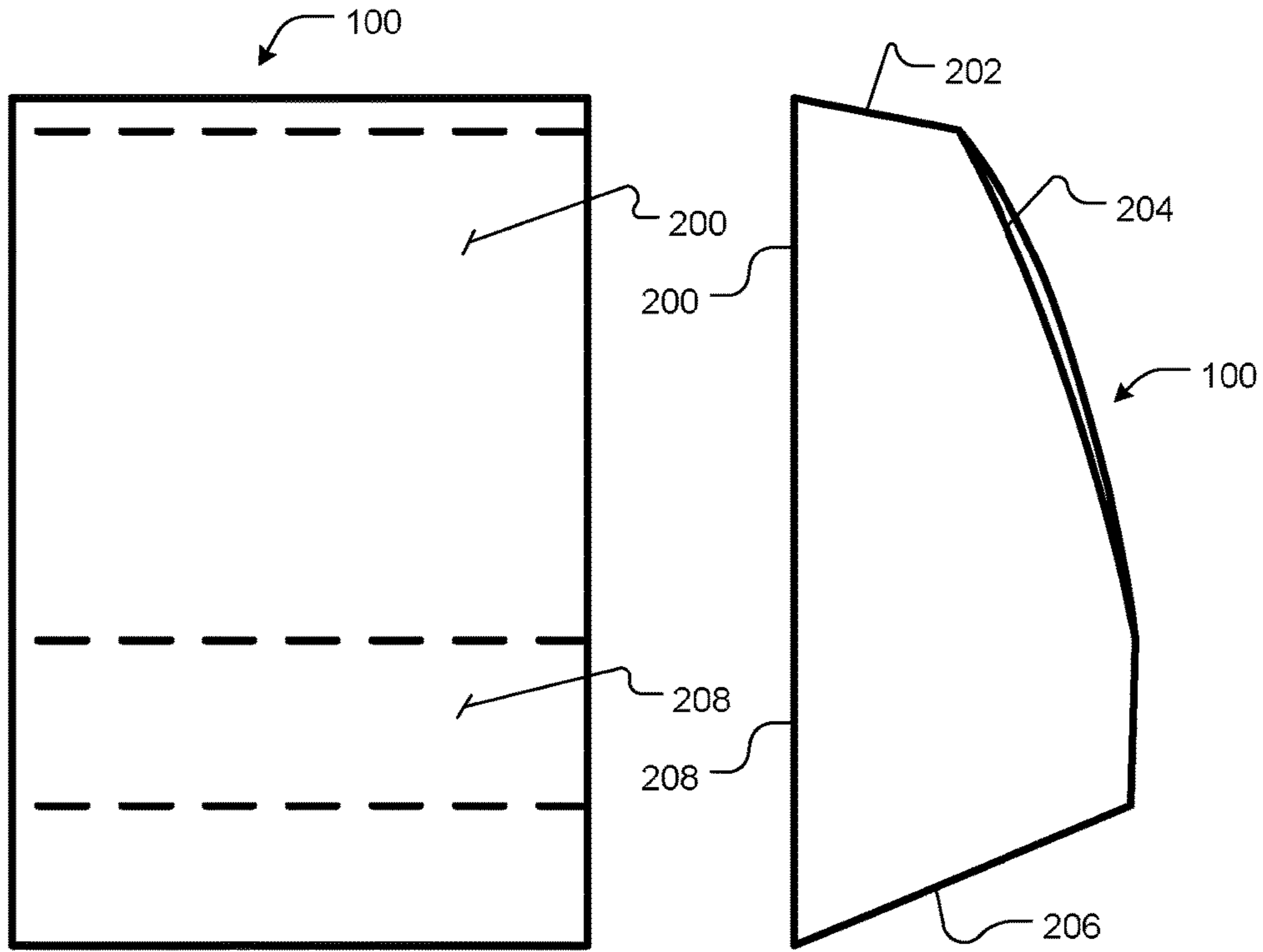
Left Side View FIG. 3
