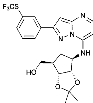
; Compound 3
