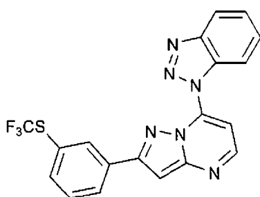
; Compound 5
