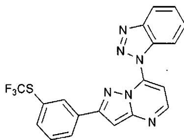
; Compound 5
