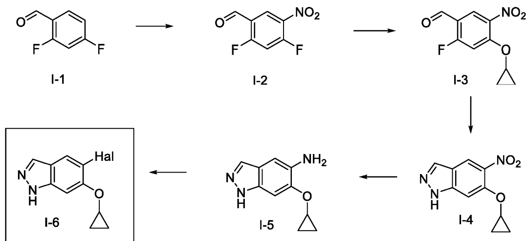
Scheme 1: Synthesis of scaffold I-6 with Hal = halide.
