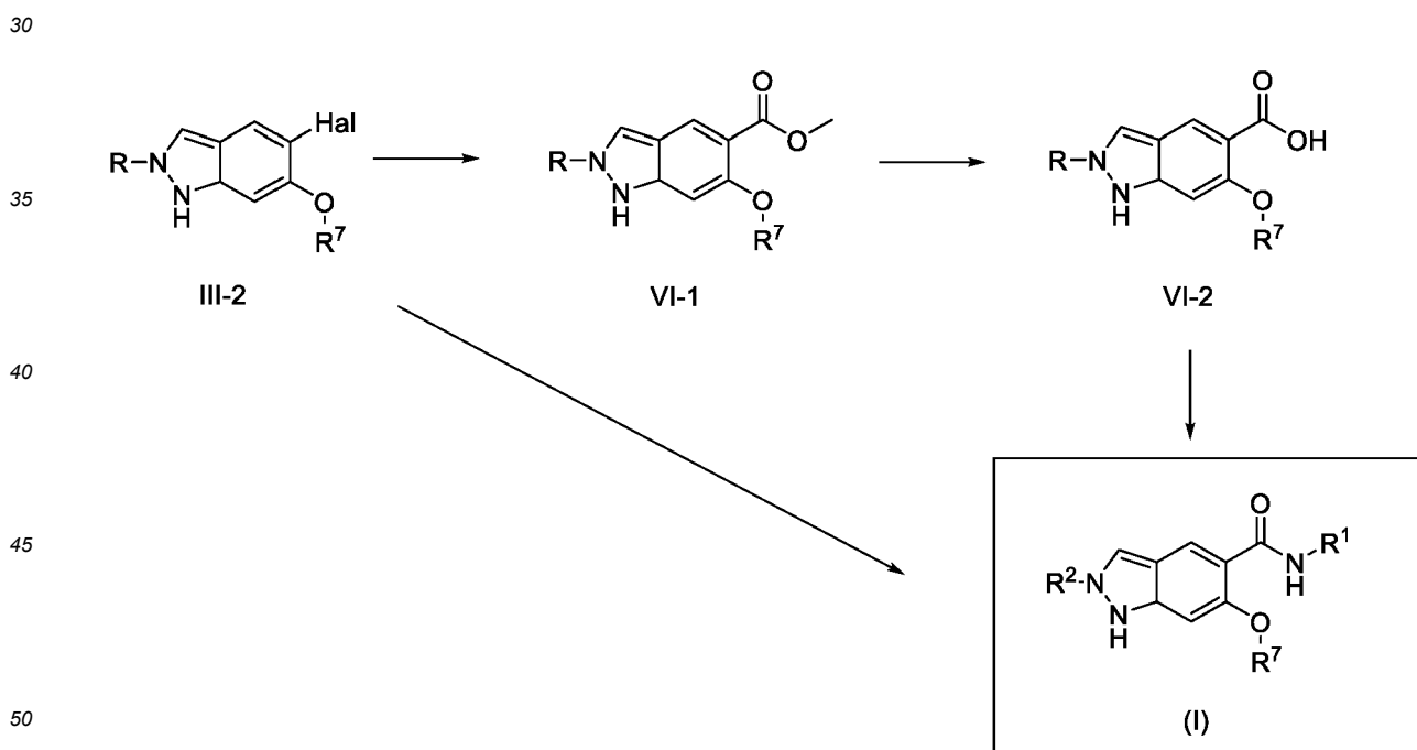
Scheme 6: General synthesis of compounds of formula (I), Method 2:
