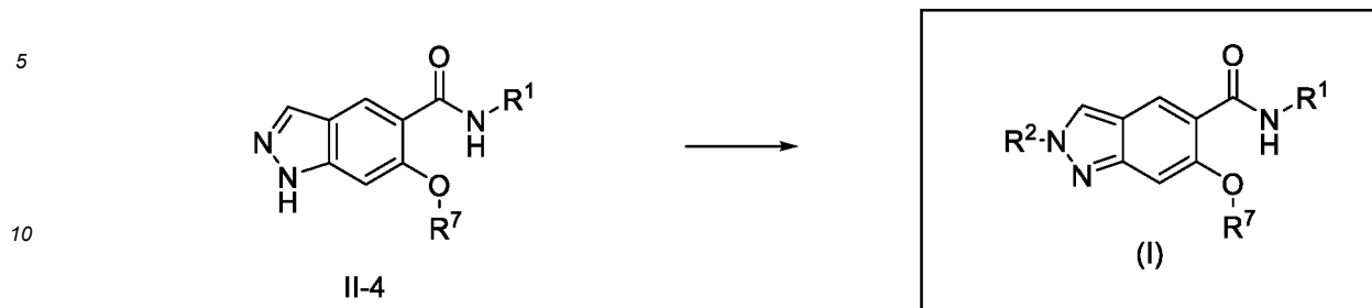
Scheme 5: General synthesis of compounds of formula (I), Method 1:
