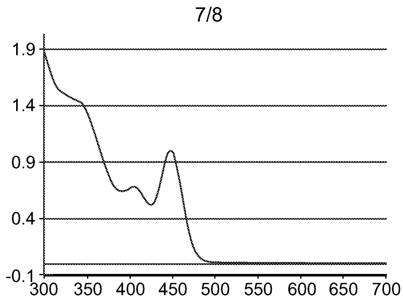
Absorption spectrum of the core material (448 nm peak, 16 nm HWHM).
