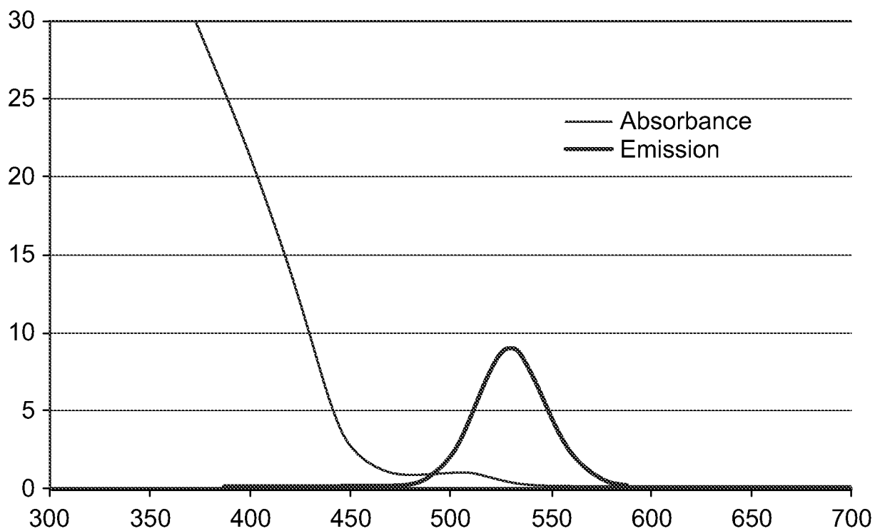
Absorption and emission spectrum of ggCdSeCS-121 (Emission Peak: 531 nm; FWHM 41 nm)
