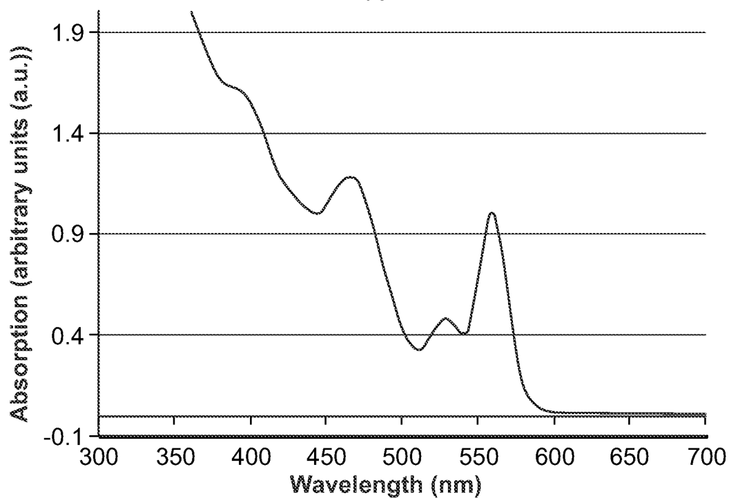
Absorption spectrum of the CdSe core material of Example IV (559 nm peak, 13 nm HWHM).
