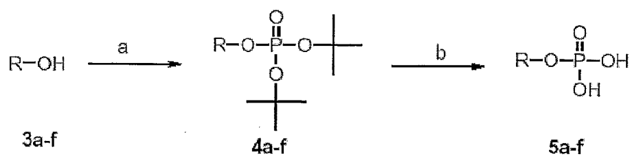
Scheme 1 a
