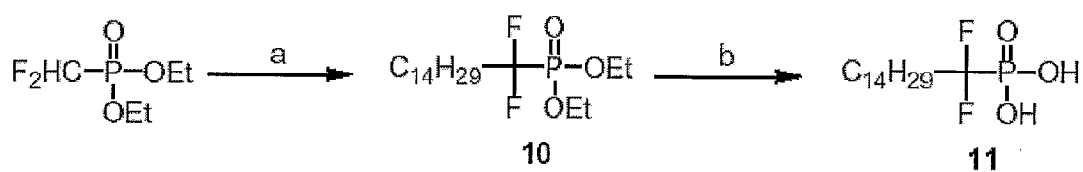
Scheme 3 a
