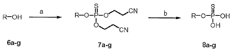
Scheme 2 a
