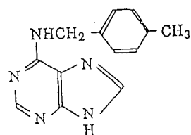
6-(4-methylbenzylamino)purine
