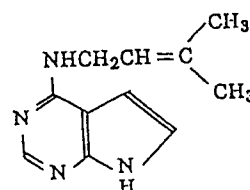
4-(3-methyl-2-butenylamino)-pyrrolo[2,3-d]pyrimidine
