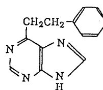
6-(2-phenethyl)purine
