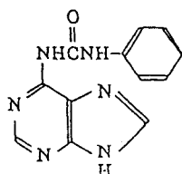
6-(phenylureido)purine
