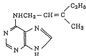
6-(3-methyl-2-pentenylamino)- purine
