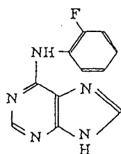
6-(2-fluorophenylamino)- purine
