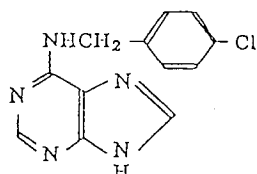
6-(4-chlorobenzylamino)purine
