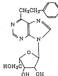
6-(2-phenethyl)-9-lyxo- furanosylpurine
