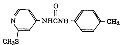
N-(2-methylthio-4-pyridyl)-N'-(4-methylphenyl)urea
