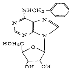
6-benzylamino-9-ribo- furanosylpurine
