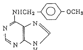
6-(4-methoxybenzylamino)- purine
