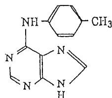
6-(4-methylphenylamino)purine
