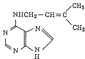
6-(3-methyl-2-butenylamino)- purine
