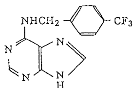
6-(4-trifluoromethylbenzyl- amino)purine
