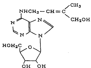
6-(4-hydroxy-3-methyl-2-butenyl amino)-9-ribofuranosylpurine
