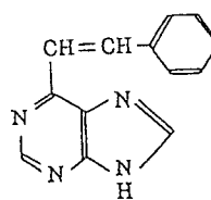
6-styryl-purine
