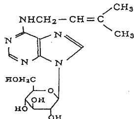
6-(3-methyl-2-butenylamino)- 9-glucosylpurine
