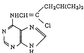
6-(2-chloro-5-methyl-1- pentenylamino)purine
