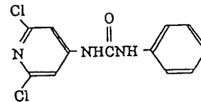
N-(2,6-dichloro-4-pyridyl)-N'-phenylurea
