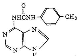
6-(4-methylphenylureido)purine
