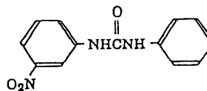
N-(3-nitrophenyl)-N'-phenylurea
