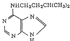
6-isoamylaminopurine
