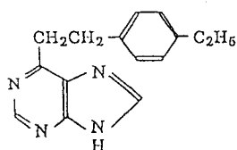
6-(4-ethyl-2-phenethyl)- purine
