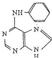
6-phenylaminopurine
