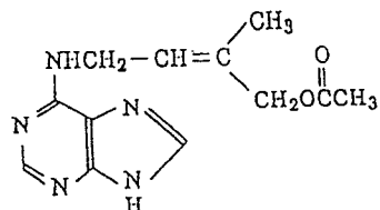
6-(4-acetoxy-3-methyl-2- butenylamino)purine
