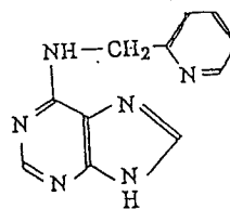
6-(2-pyridylmethylamino)- purine
