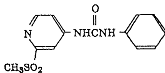
N-(2-methylsulfonyl-4-pyridyl)-N'-phenylurea
