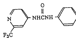
N-(2-trifluoromethyl-4-pyridyl)-N'-phenylurea
