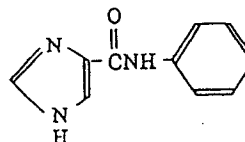
4-imidazolecarbanilide
