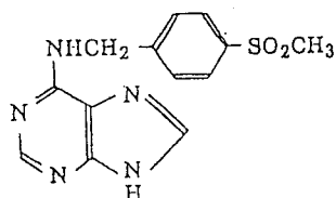
6-(4-methylsulfonylbenzyl- amino)purine
