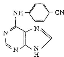
6-(4-cyanophenylamino)purine
