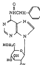
6-phenylureido-9-glucosyl- purine
