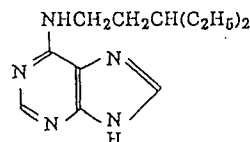
6-(3-ethylpentylamino)purine
