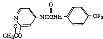
N-(2-acetoxy-4-pyridyl)-N'-(4-trifluoromethylphenyl)urea
