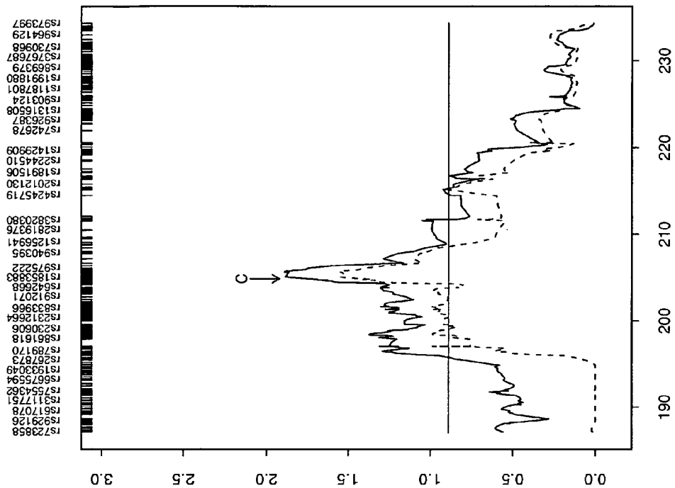
Chromosome 1: 533 SNPs (H-clust 0.5)
