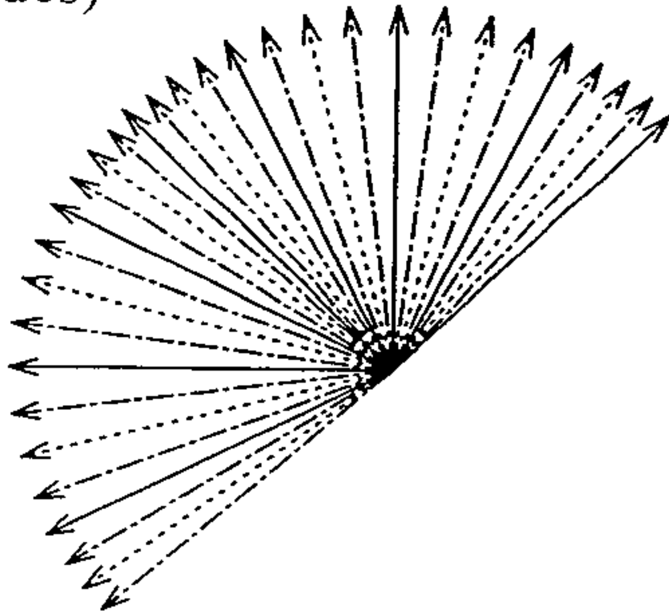
Directional Prediction in Case of N=33 (32 Modes)
