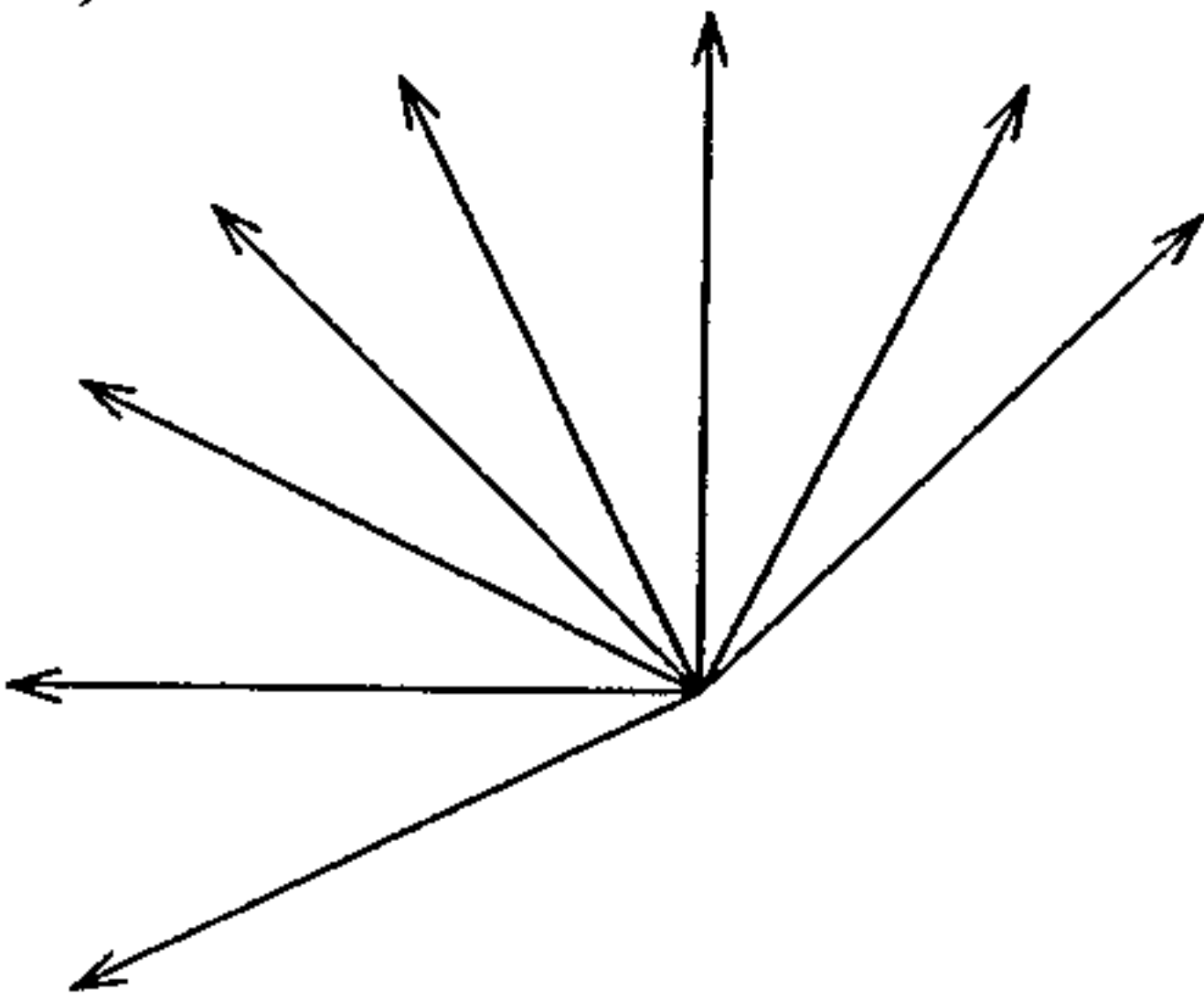
Directional Predictions in Case of N=9 (8 Modes)
