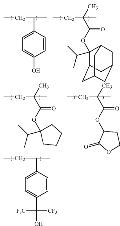
Example 2 [Synthesis of Resin A2]
