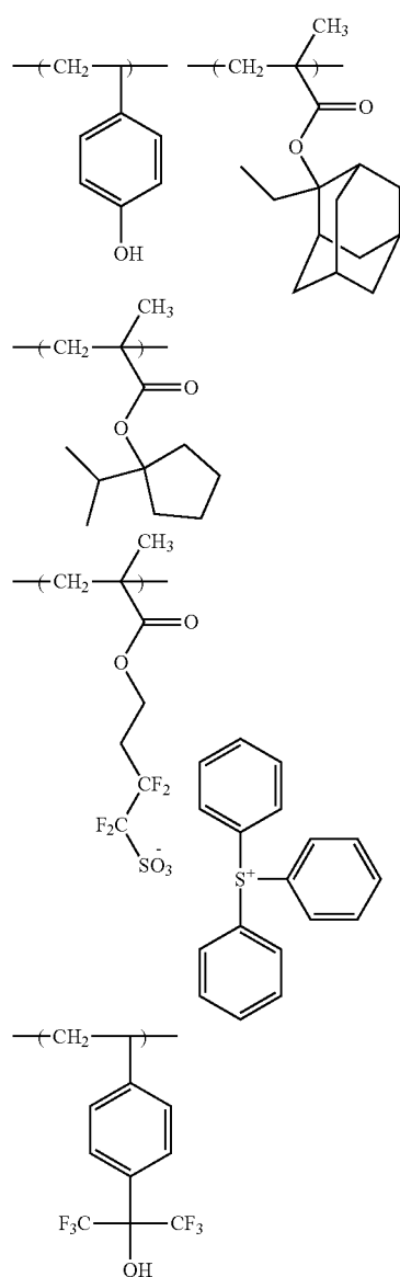
Example 5 [Synthesis of Resin A5]
