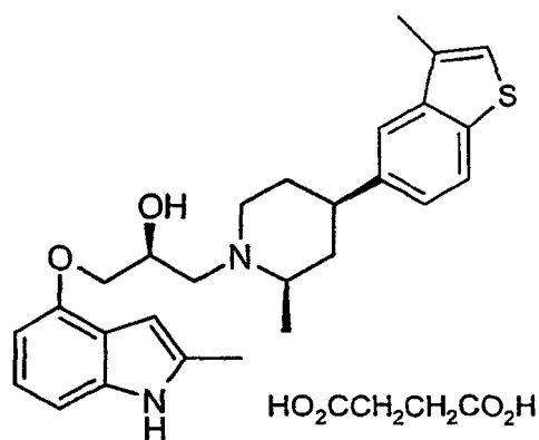
Isomer 1
