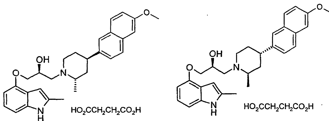
isomers 3 and 4
