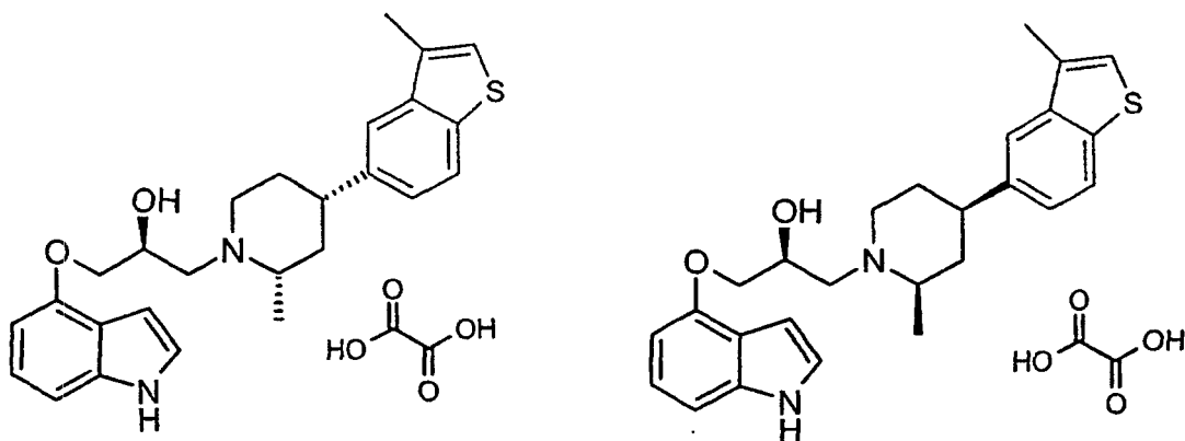
isomers 1 and 2
