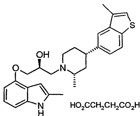
Isomer 2
