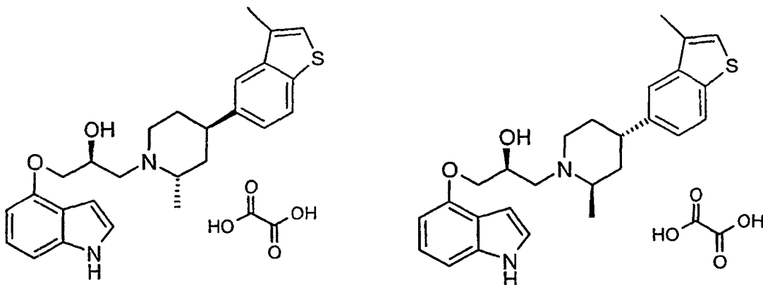
isomers 3 and 4
