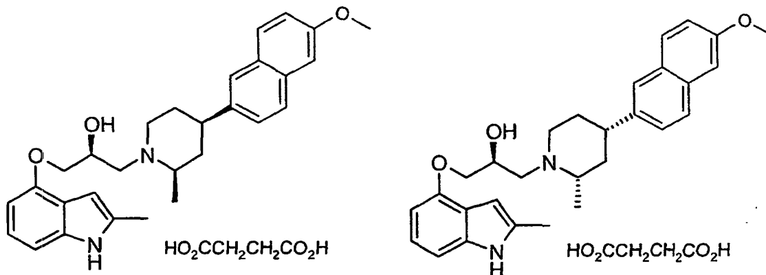
isomers 1 and 2
