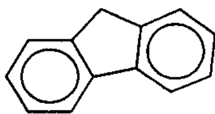
fluorene MW = 166
