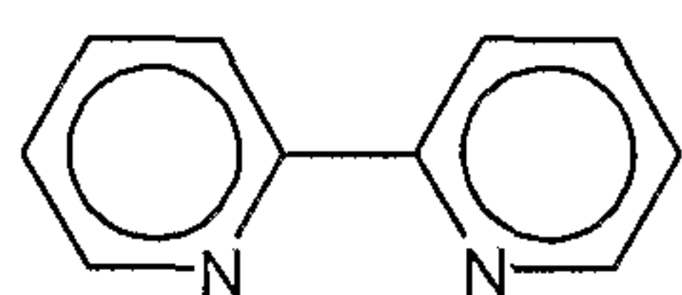
2,2' dipyridyl MW = 156
