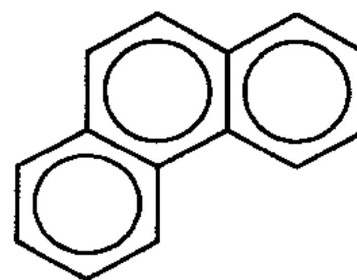
phenanthrene MW = 178
