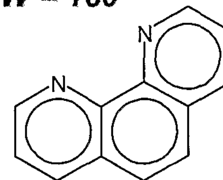
1, 10' phenanthroline MW = 180
