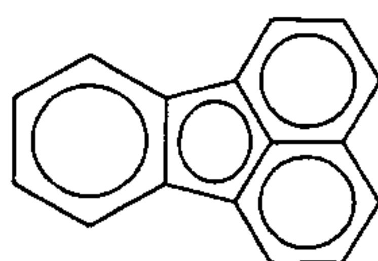
fluoranthene MW = 202
