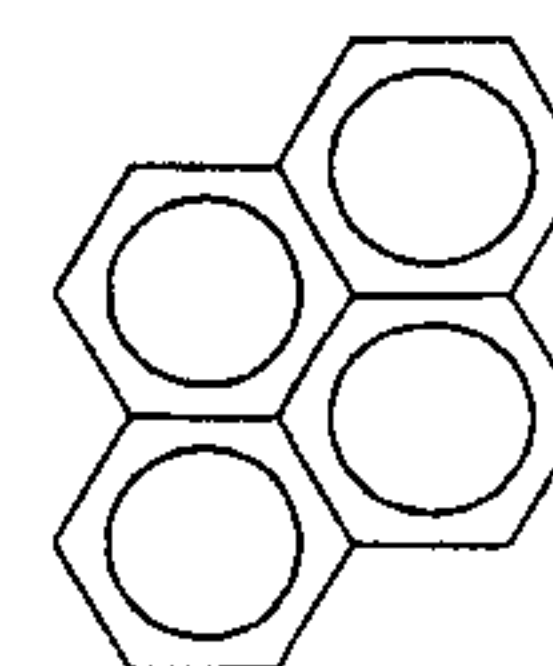
pyrene MW = 202
