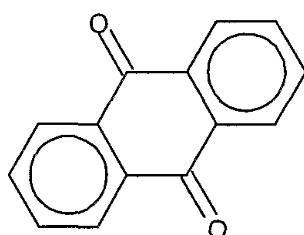
anthraquinone MW = 208
