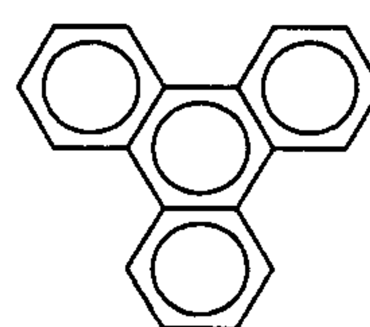
triphenylene MW = 228
