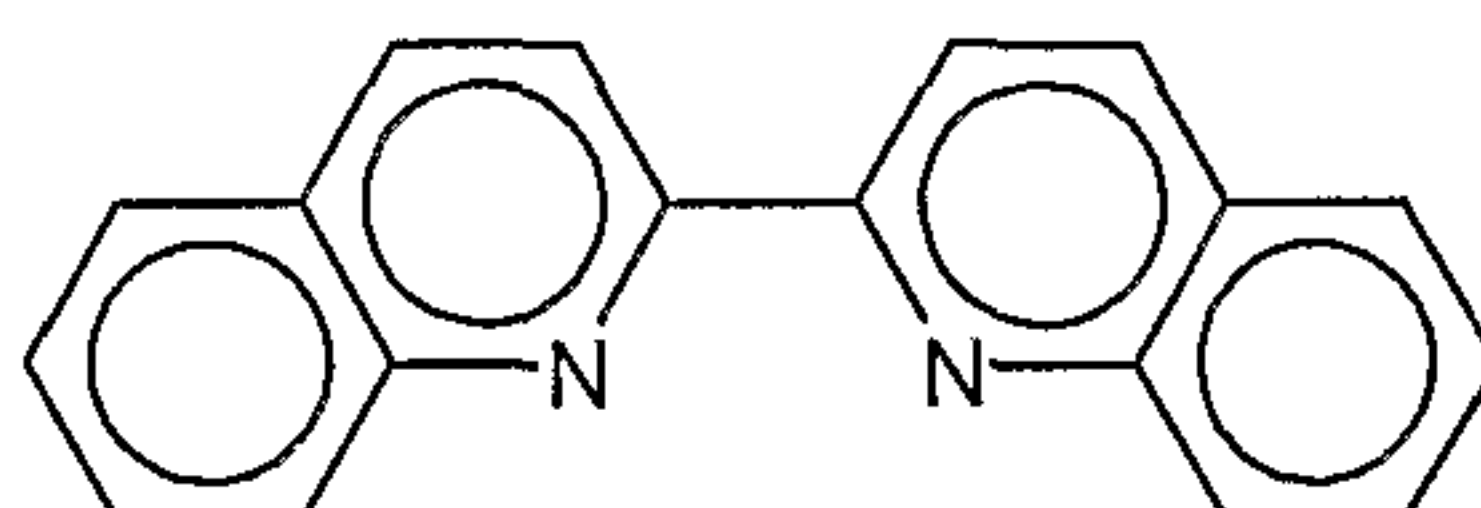
2,2' biquinoyline MW = 256
