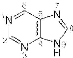
Purine
