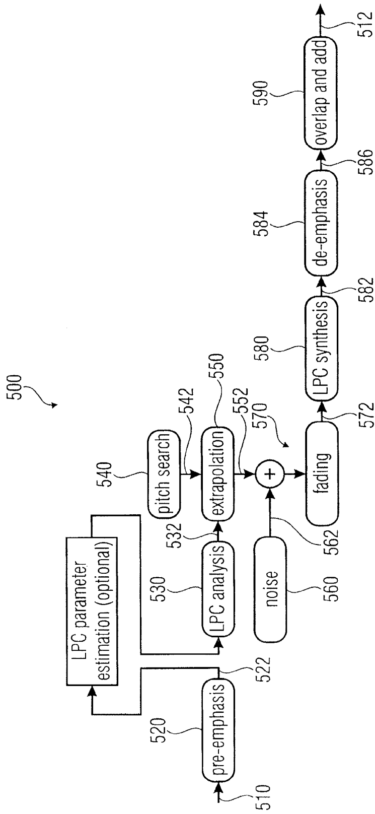
Time domain concealment overview for transform decoder FIG 5
