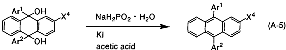
Compound I
