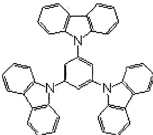
[Chemical Formula 44]
