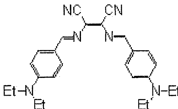
[Chemical Formula 72]
