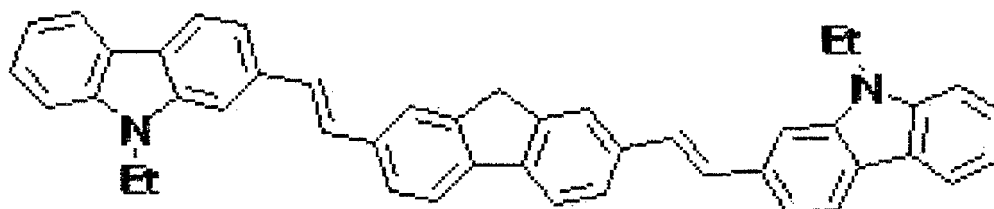
[Chemical Formula 65]
