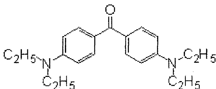
[Chemical Formula 54]
