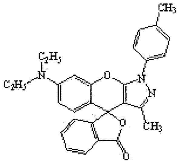
[Chemical Formula 106]
