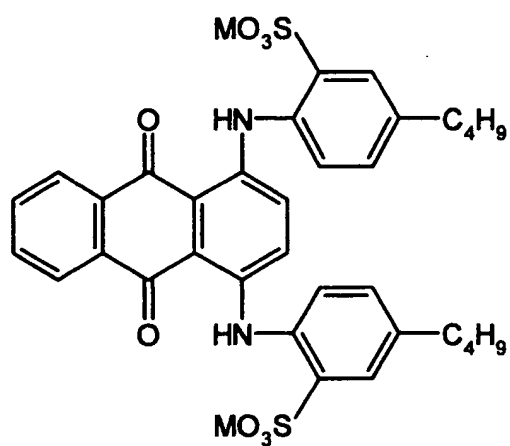
Compound Example No. 3-2
