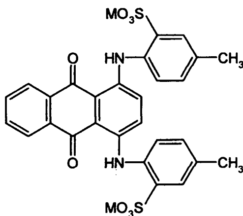
Compound Example No. 3-1
