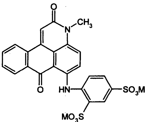
Compound Example No. 4-3
