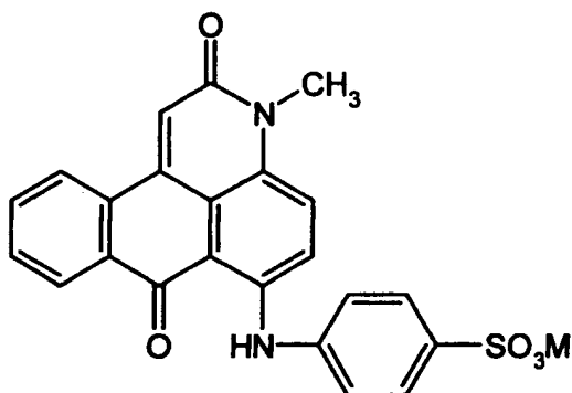
Compound Example No. 4-1
