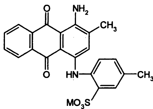
Compound Example No. 3-7
