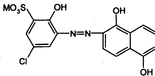
Compound Example No. 1-6
