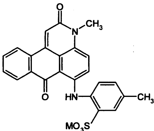
Compound Example No. 4-2
