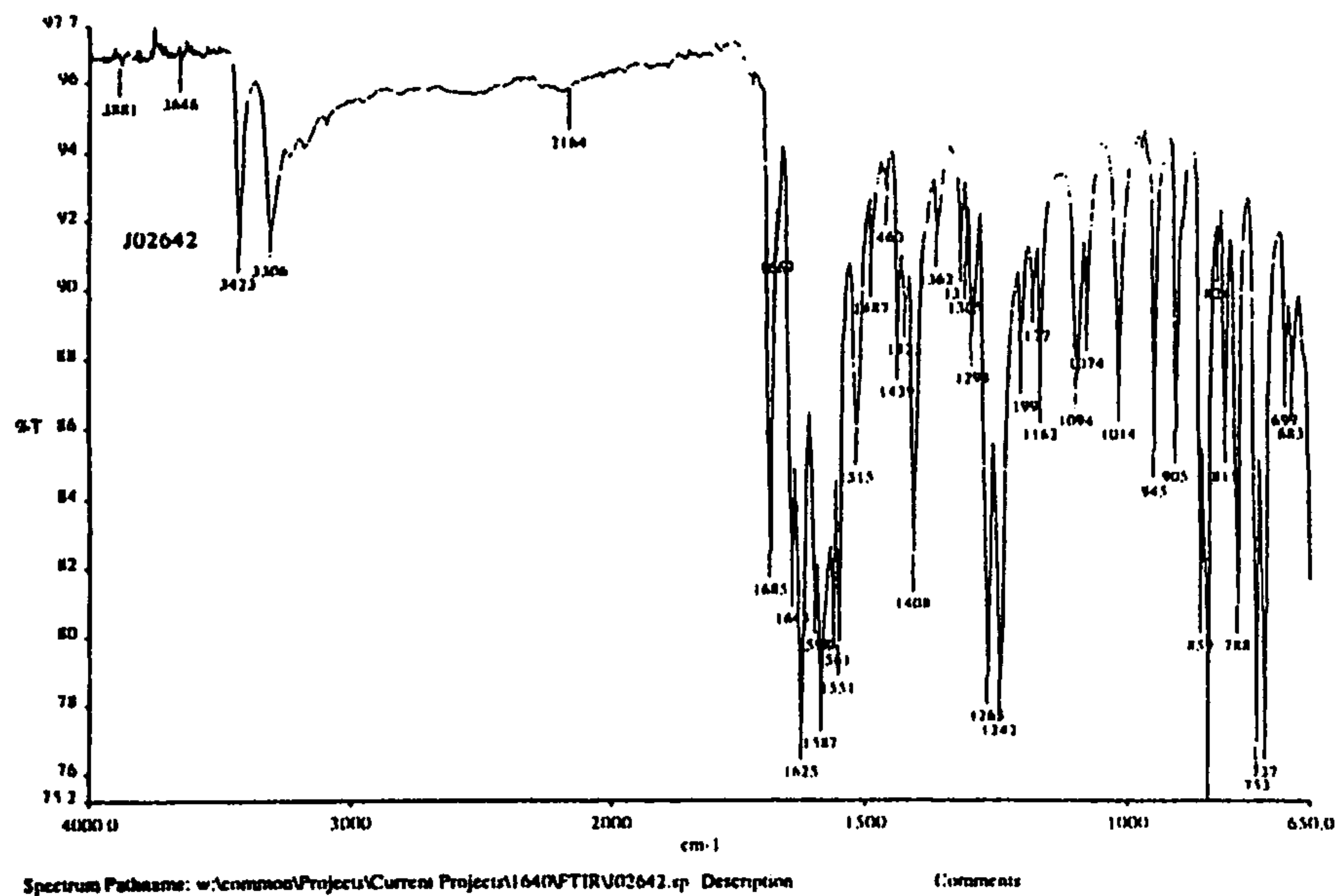
Figure 15-4 FT-IR of J02642, Pattern 1 as supplied
