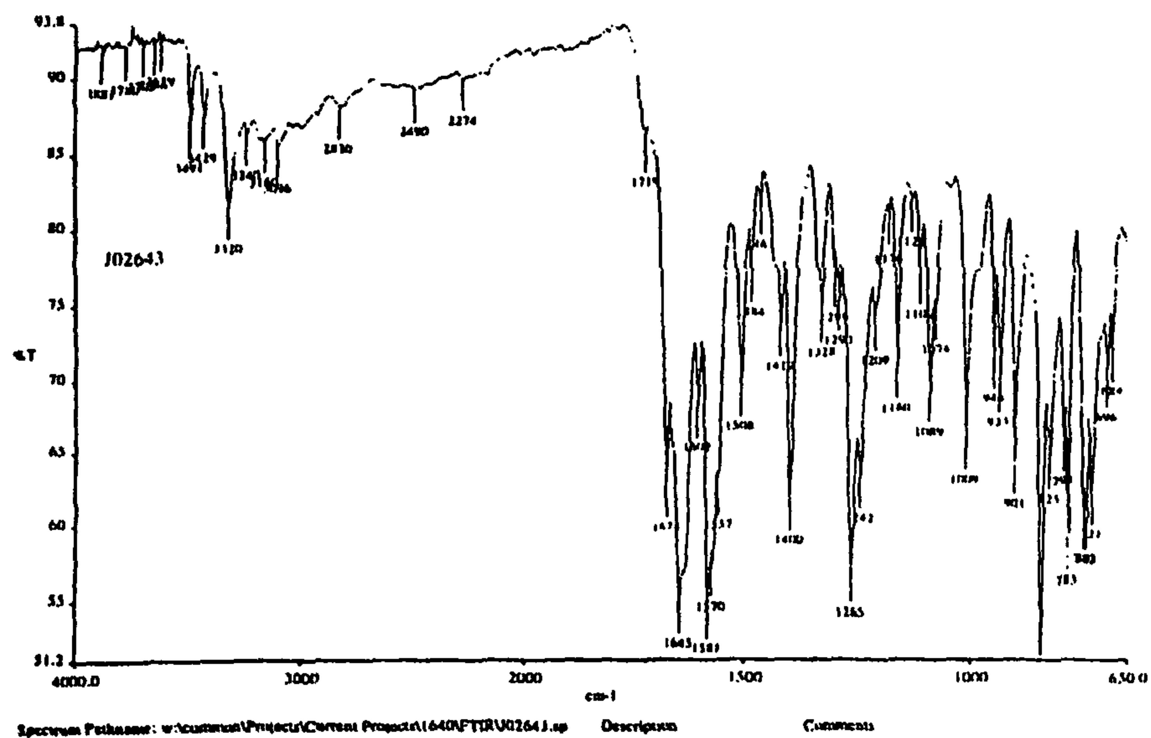
Figure 15-5 FT-IR of J02643, Pattern 2 as supplied
