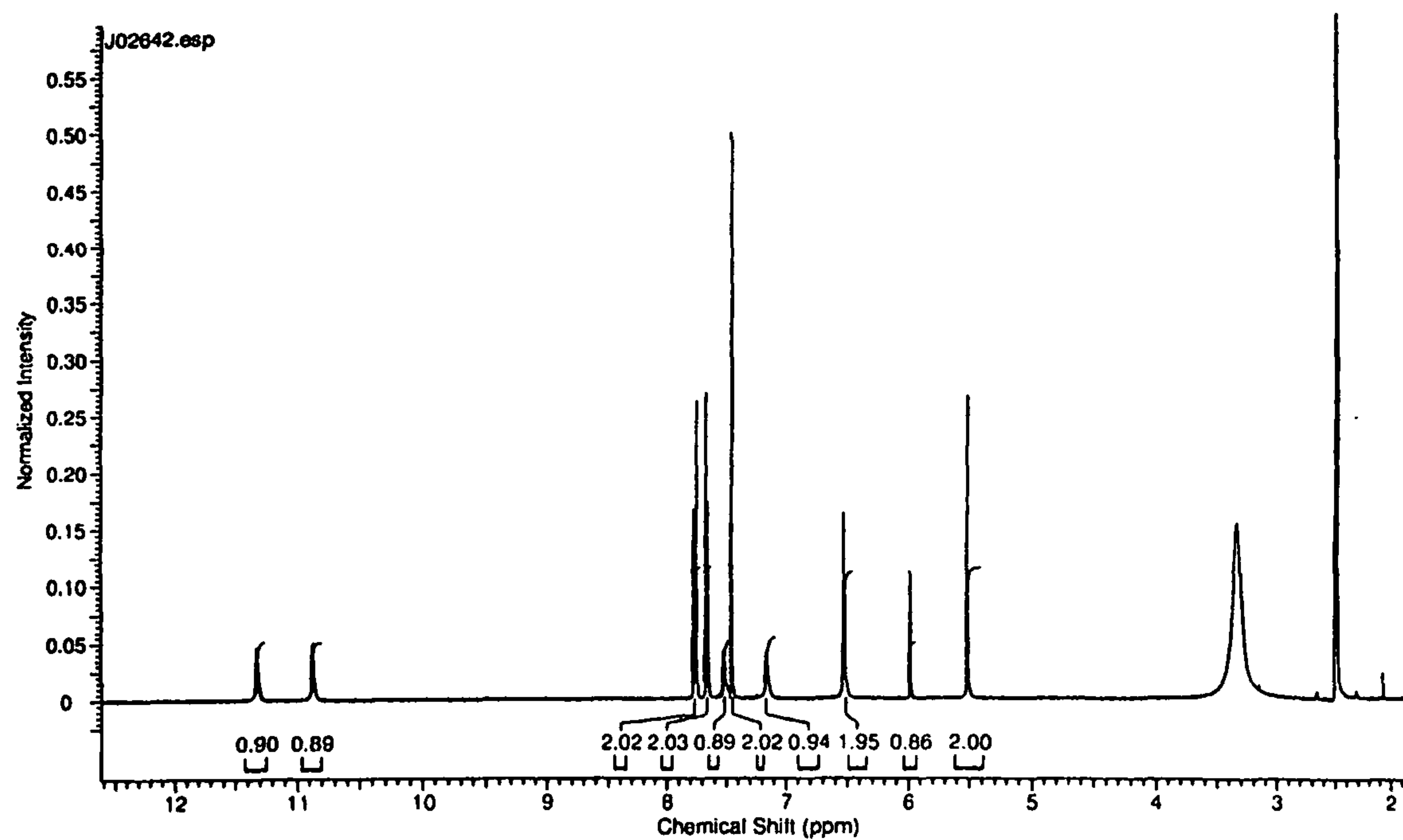
^1\text{H} NMR analysis of J02642
