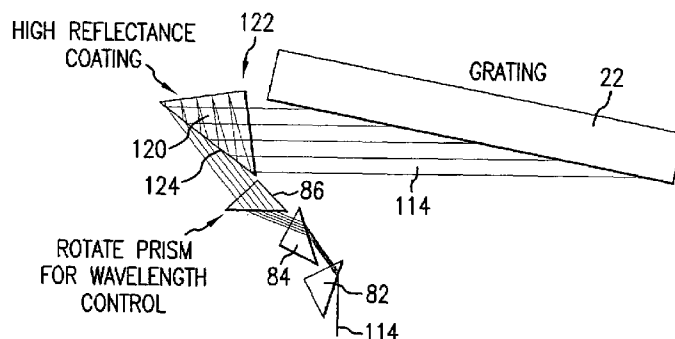
OPTICAL DESIGN FOR COMPACT LNM ROBERT BERGSTEDT 5/27/04
