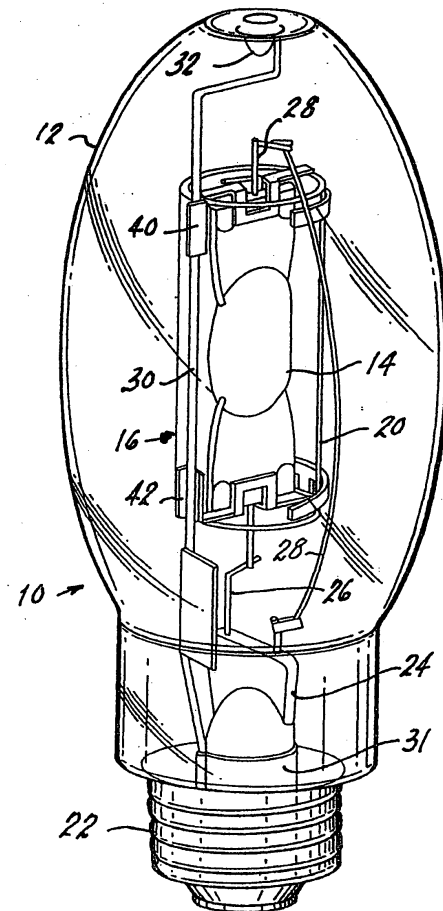
FIG. 1 PRIOR ART
