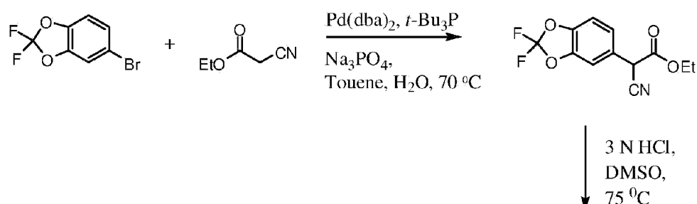
Scheme 2. Alternative synthesis of the acid chloride moiety.
