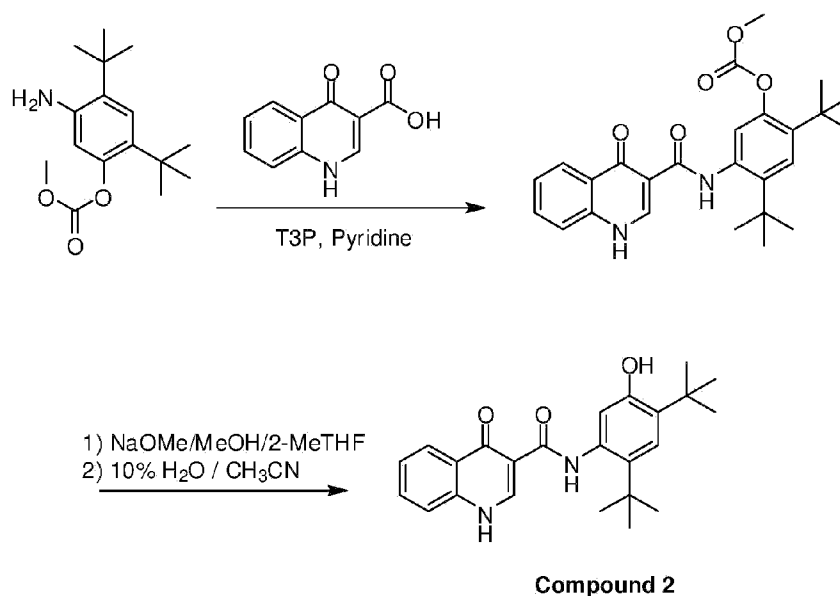
Scheme 7: Coupling of the 4-oxo-dihydroquinoline carboxylic acid moiety with the amine moiety.
