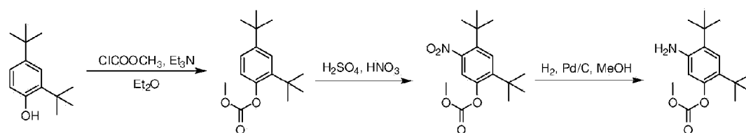
Scheme 7: Coupling of the 4-oxo-dihydroquinoline carboxylic acid moiety with the amine moiety.
