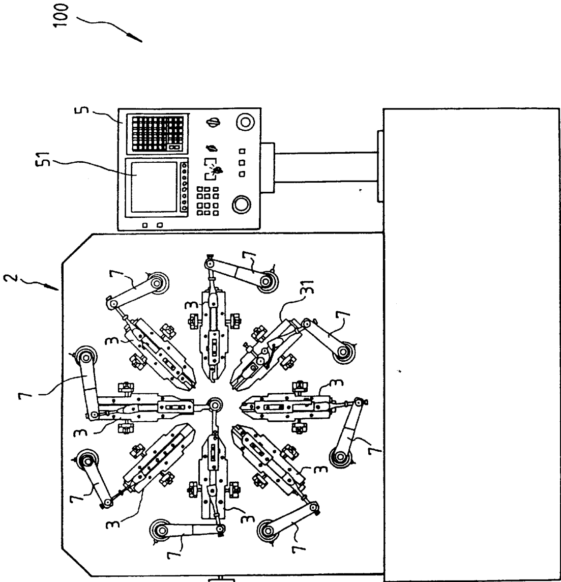
FIG.7 PRIOR ART
