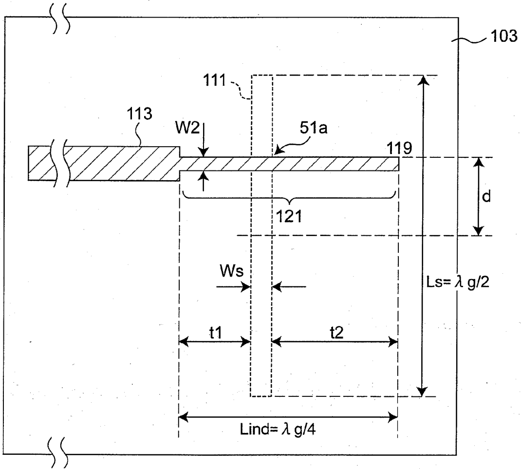
Fig.36 PRIOR ART
