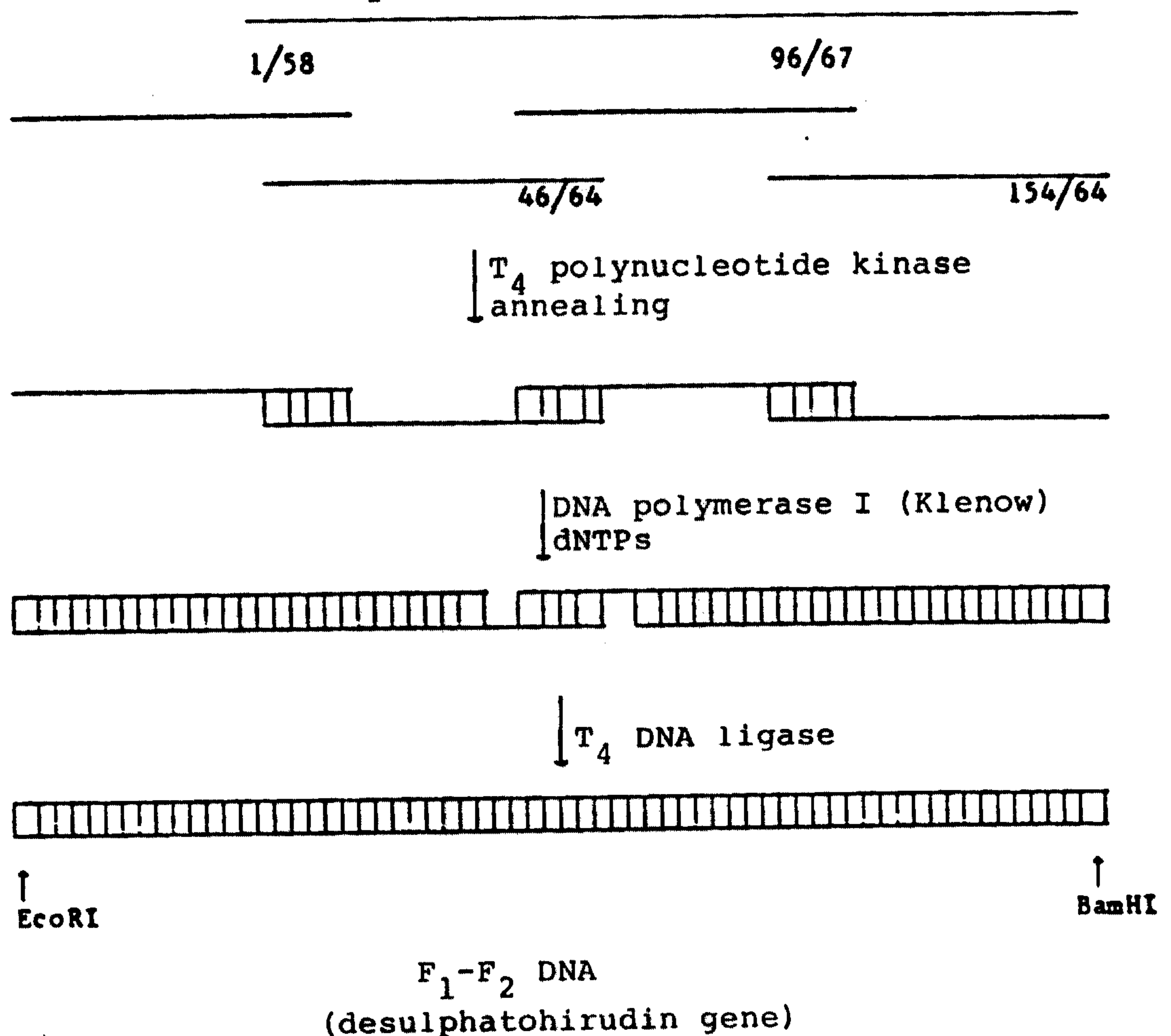
Scheme 6: Manufacture of the hirudin gene from the four synthetic fragments
