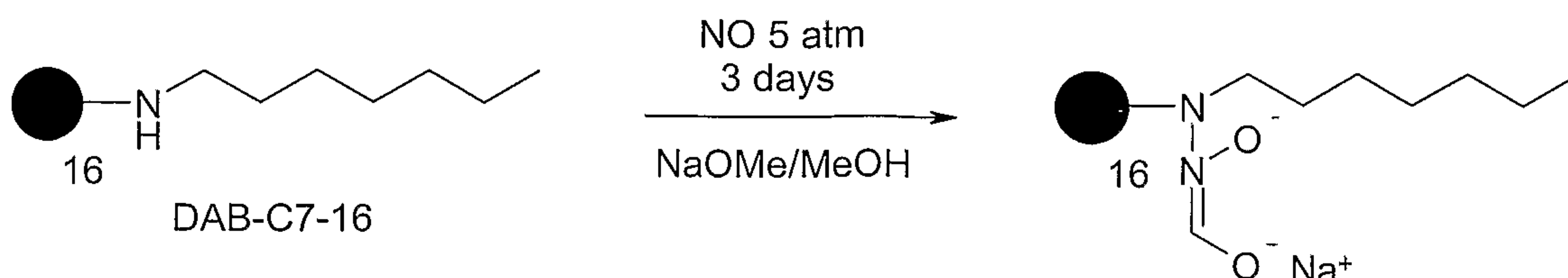
Scheme 5. Preparation of DAB-C7-16 diazeniumdiolate.
