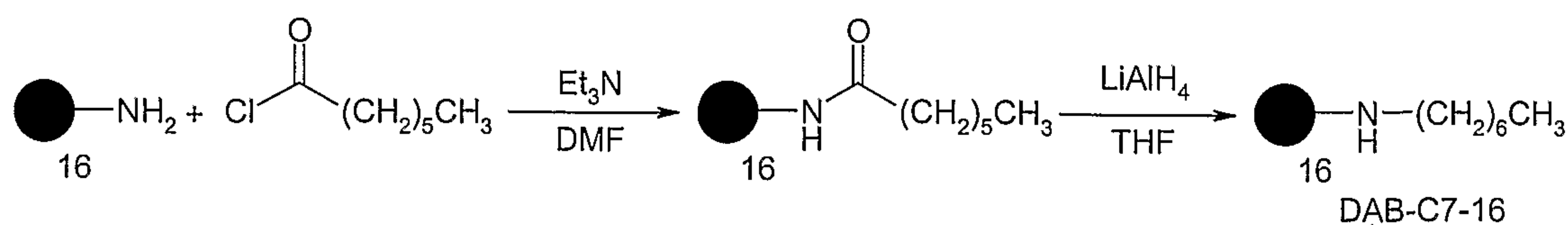
Scheme 4. Preparation of DAB-C7-16.
