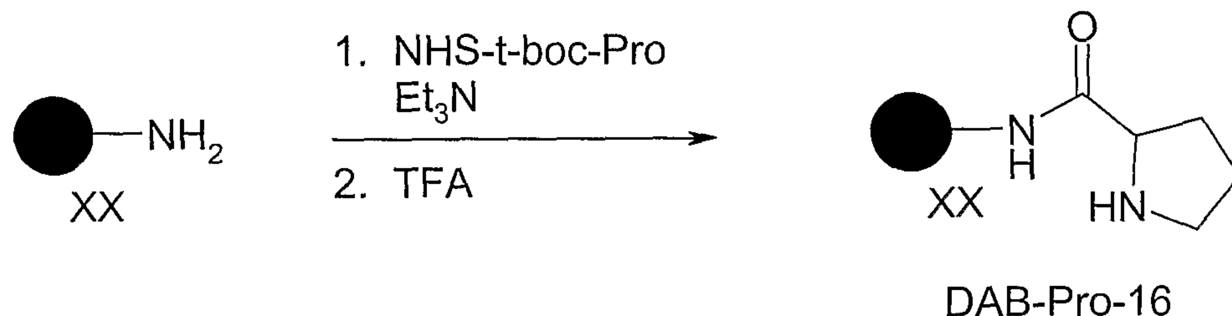
Scheme 7. Preparation of DAB-Pro-16.
