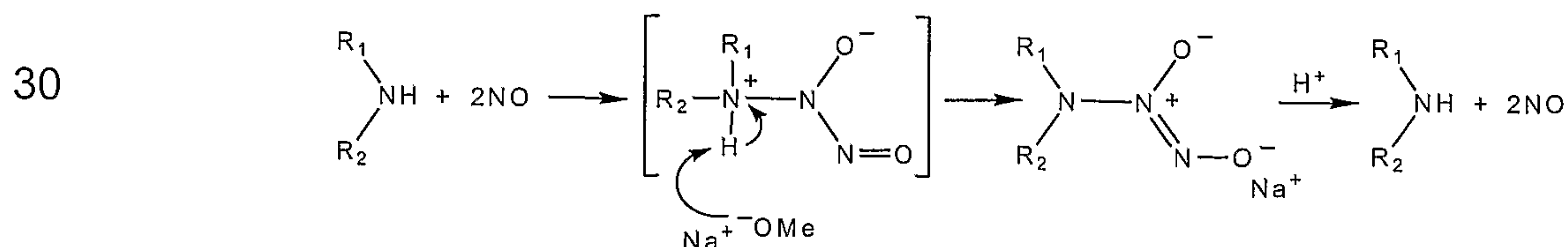
Scheme 1. Synthesis and NO-release from N -diazoniumdiolates.
