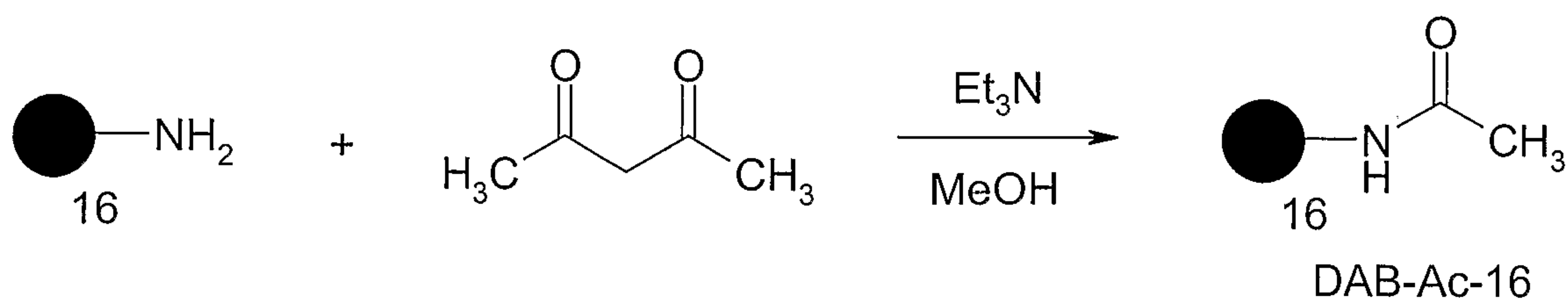
Scheme 6. Preparation of DAB-Ac-16.
