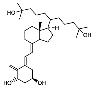
1,25-Dihydroxy-21- (3-hydroxy-3-methyl-butyl)- 5,6-trans-cholecalciferol
