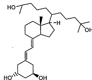
1,25-Dihydroxy-21-(3-hydroxy-3-methyl-butyl)-19-nor-cholecalciferol
