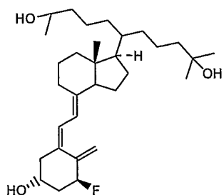
1 \alpha -Fluoro-25-hydroxy-21-(3-hydroxy-3-methyl-butyl)-cholecalciferol
