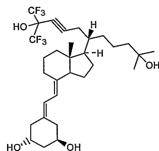
1,25-Dihydroxy-21- (3-hydroxy-3-trifluoromethyl-4- trifluoro-butynyl)-20S-19-nor-cholecalciferol
