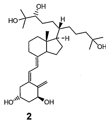
1,25-Dihydroxy-21- (2R,3-dihydroxy-3-methyl- butyl)- -20S-cholecalciferol
