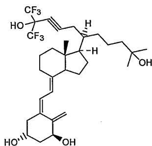
1,25-Dihydroxy-21-(3-hydroxy-3-trifluoromethyl-4-trifluorobutynyl)-20R-cholecalciferol
