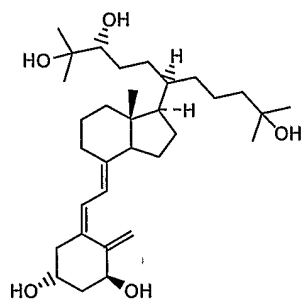
1,25-Dihydroxy-21- (2R,3-dihydroxy-3-methyl-butyl)- -20R-cholecalciferol
