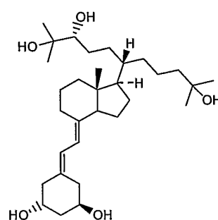
1,25-Dihydroxy-21-(2R,3-dihydroxy-3-methyl-butyl)-20S-19-nor-cholecalciferol
