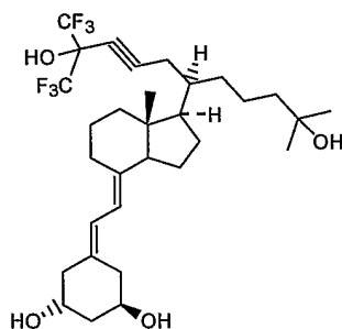
1,25-Dihydroxy-21- (3-hydroxy-3-trifluoromethyl-4-trifluoro- butynyl)-20R-19-nor-cholecalciferol
