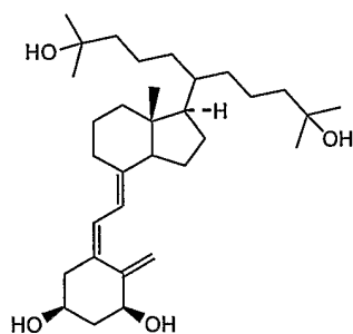
1,25-Dihydroxy-21- (3-hydroxy-3-methyl-butyl)-3- epi-cholecalciferol
