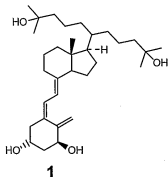
1,25-Dihydroxy-21- (3-hydroxy-3-methyl- butyl)-cholecalciferol
