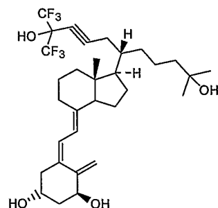
1,25-Dihydroxy-21- (3-hydroxy-3-trifluoromethyl-4- trifluoro-butynyl)-20S-cholecalciferol
