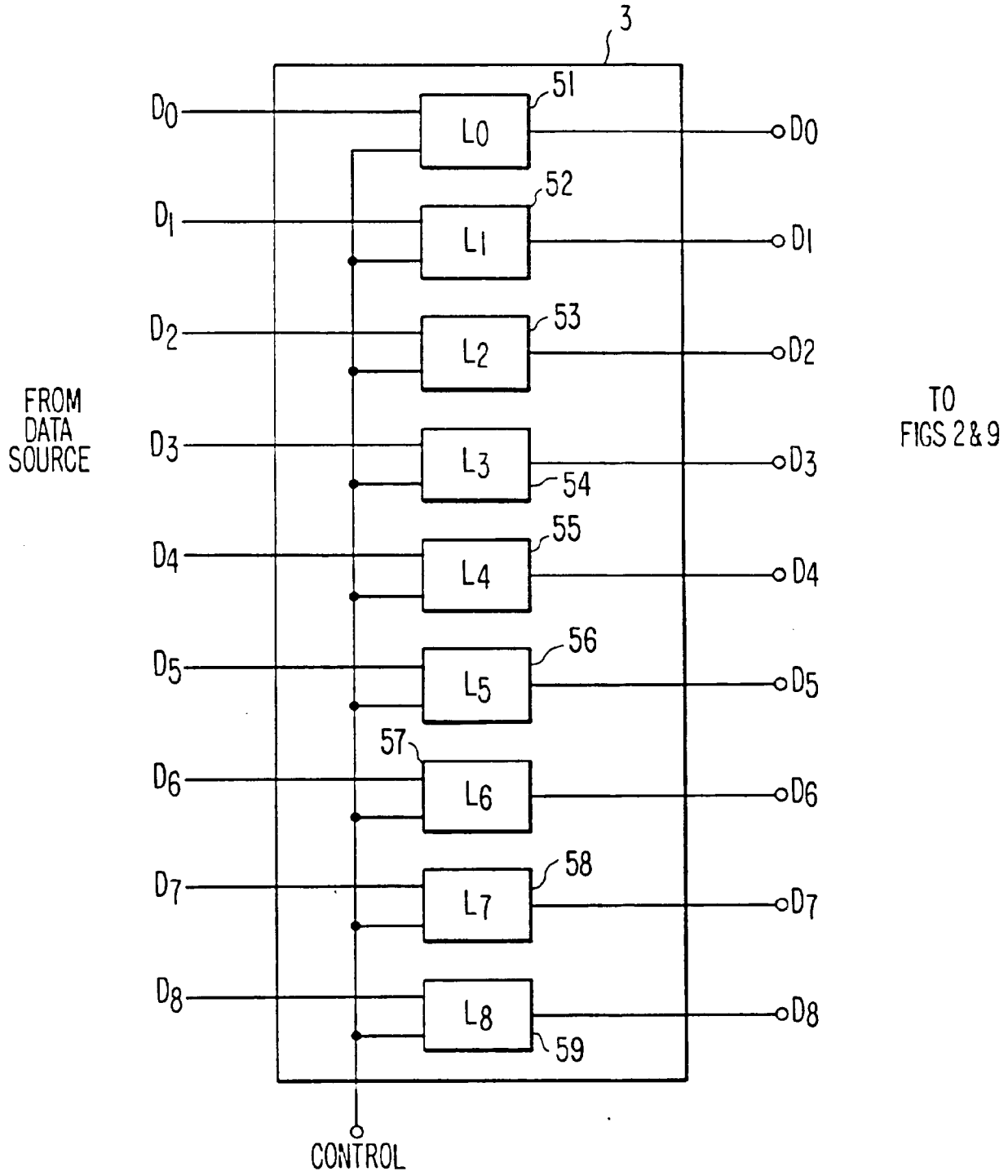
FIG. 7. CTGU-2 REGISTER
