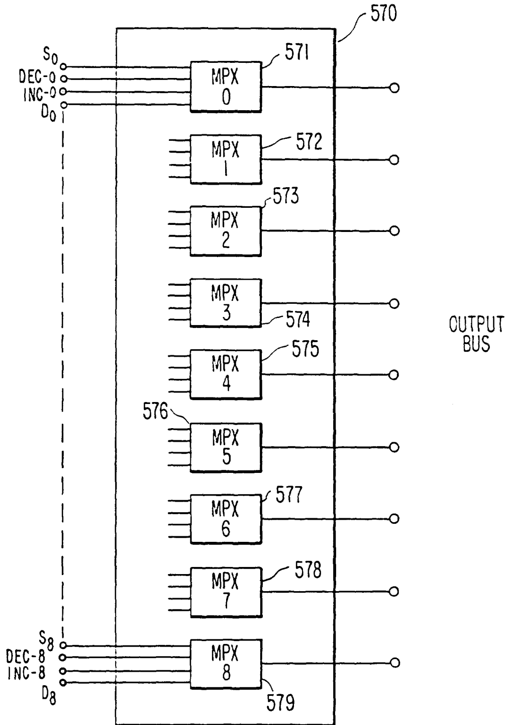
MULTIPLEXOR UNIT
