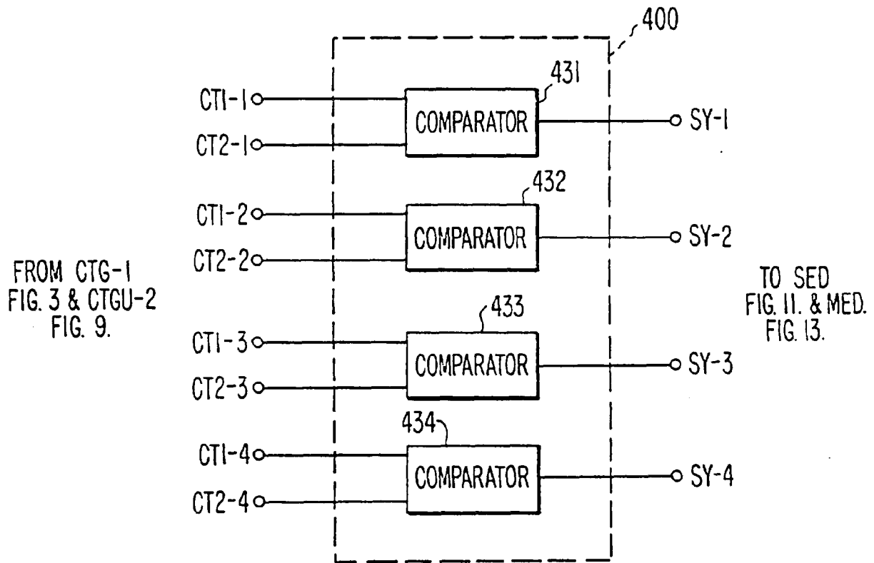
CHECK TRIT COMPARATOR UNIT
