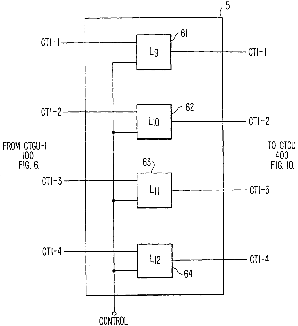
FIG. 8. CTGU-1 REGISTER
