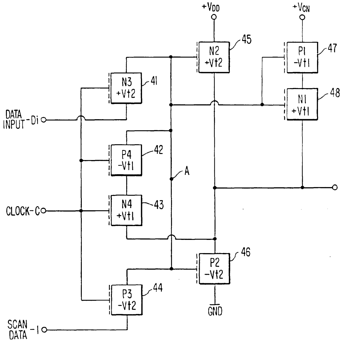
TRINARY LATCH
