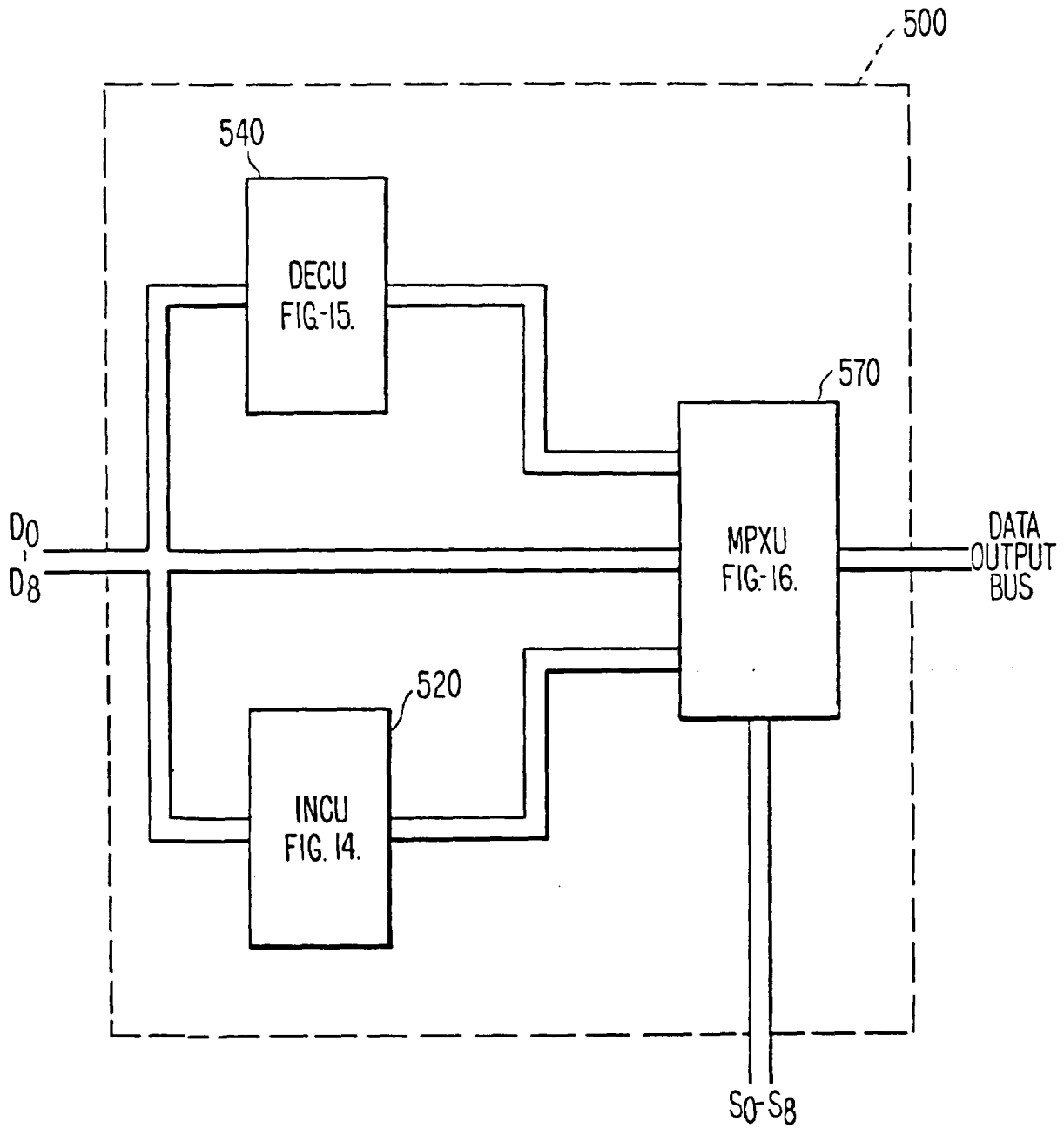
FIG. 2. DATA CORRECTOR
