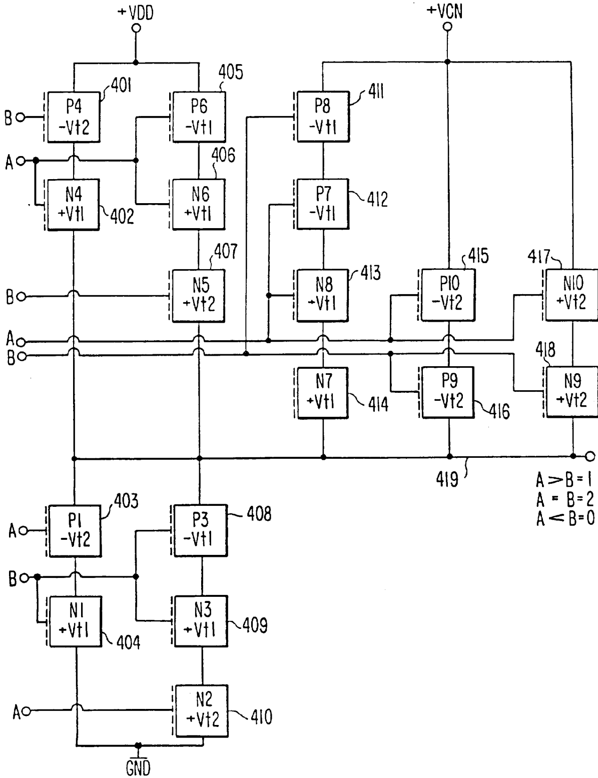
FIG. 10A. TRINARY LOGIC COMPARATOR
