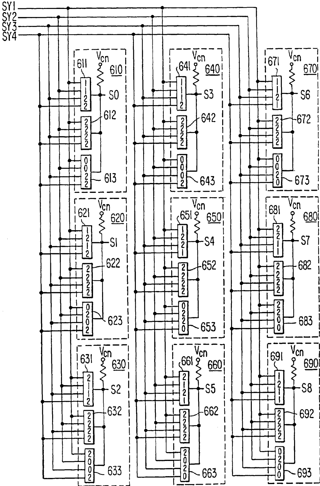
SINGLE ERROR DETECTOR 600
