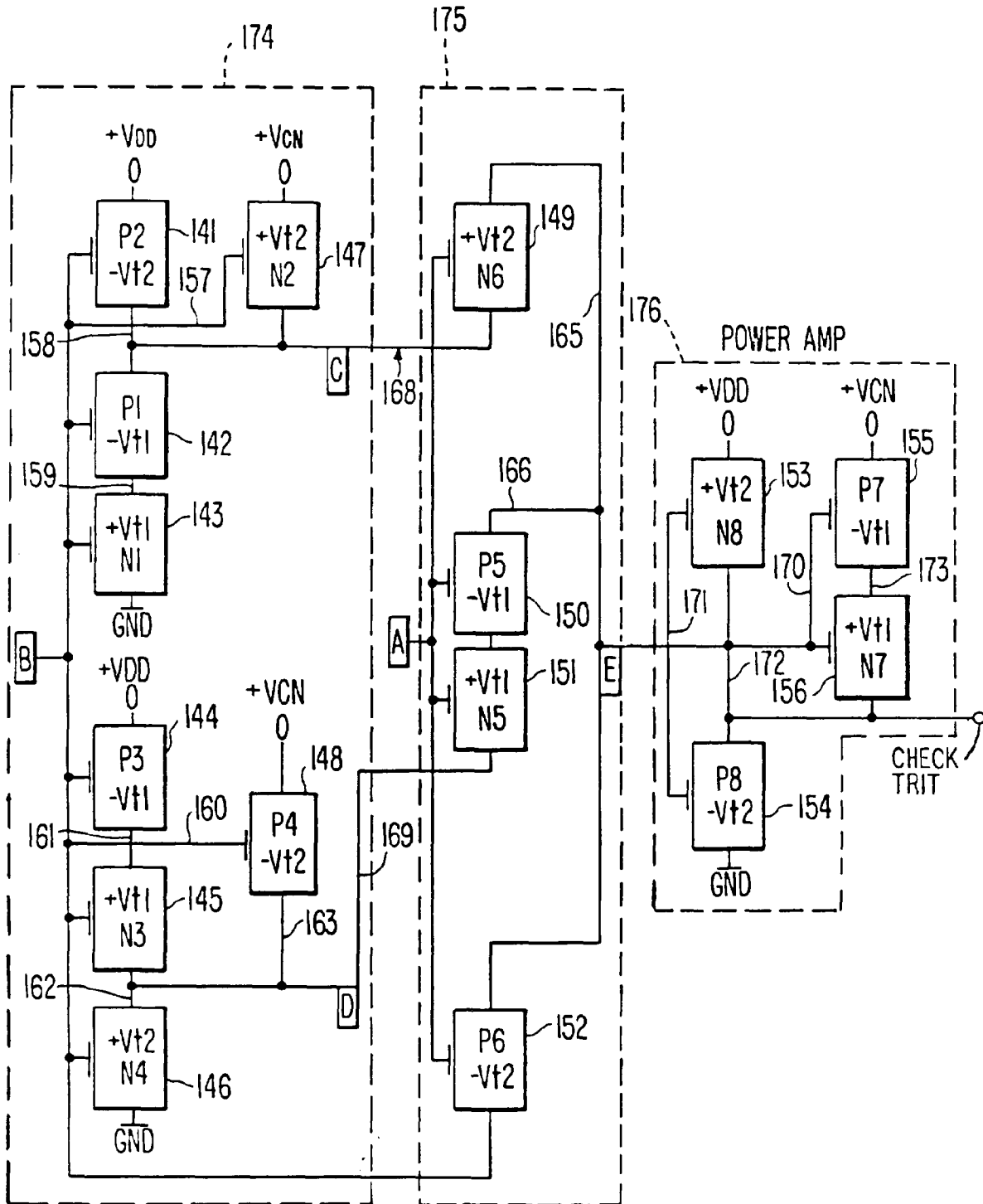
FIG. 3. TRINARY CHECK TRIT GENERATOR
