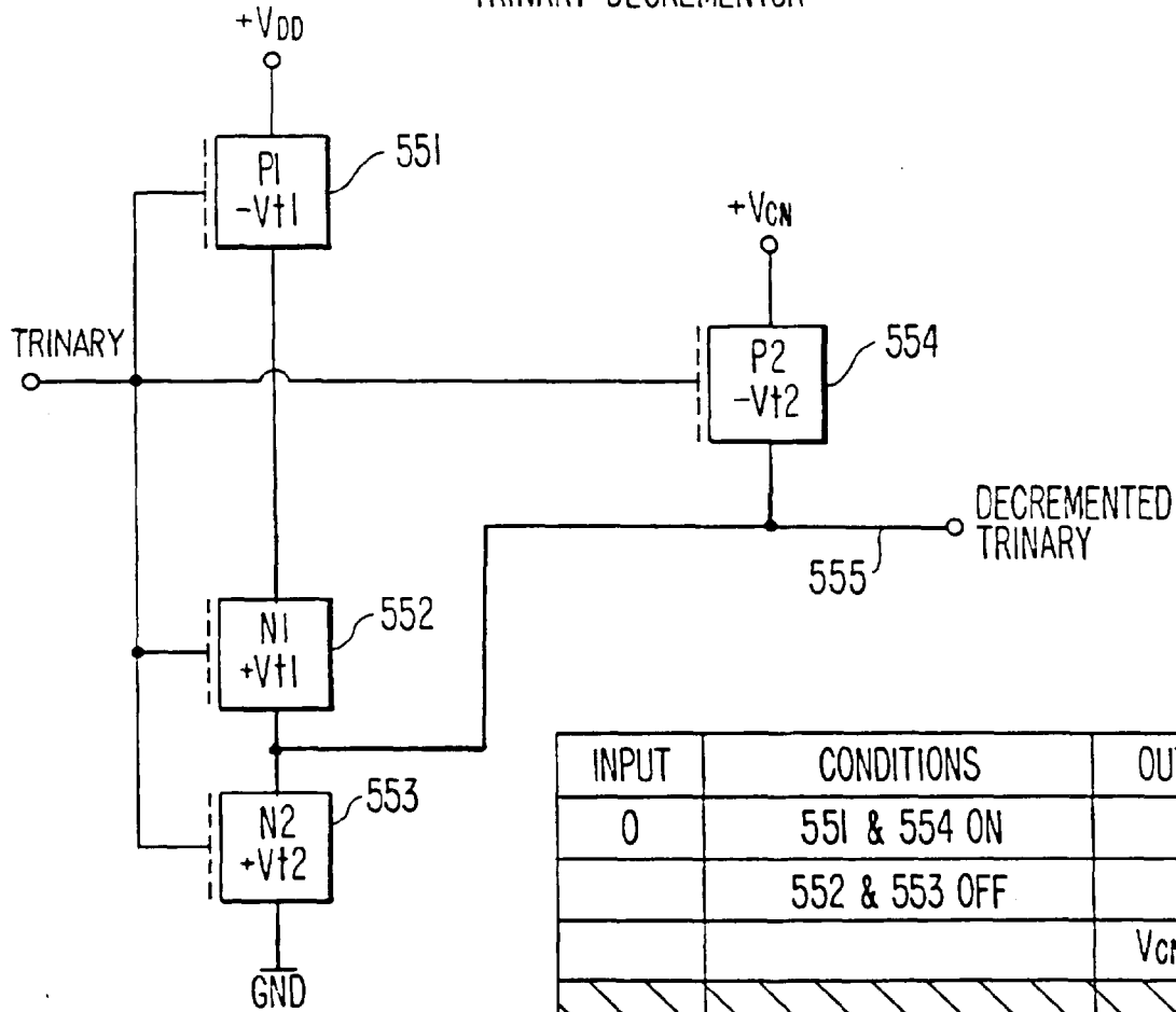
TRINARY DECREMOTOR
