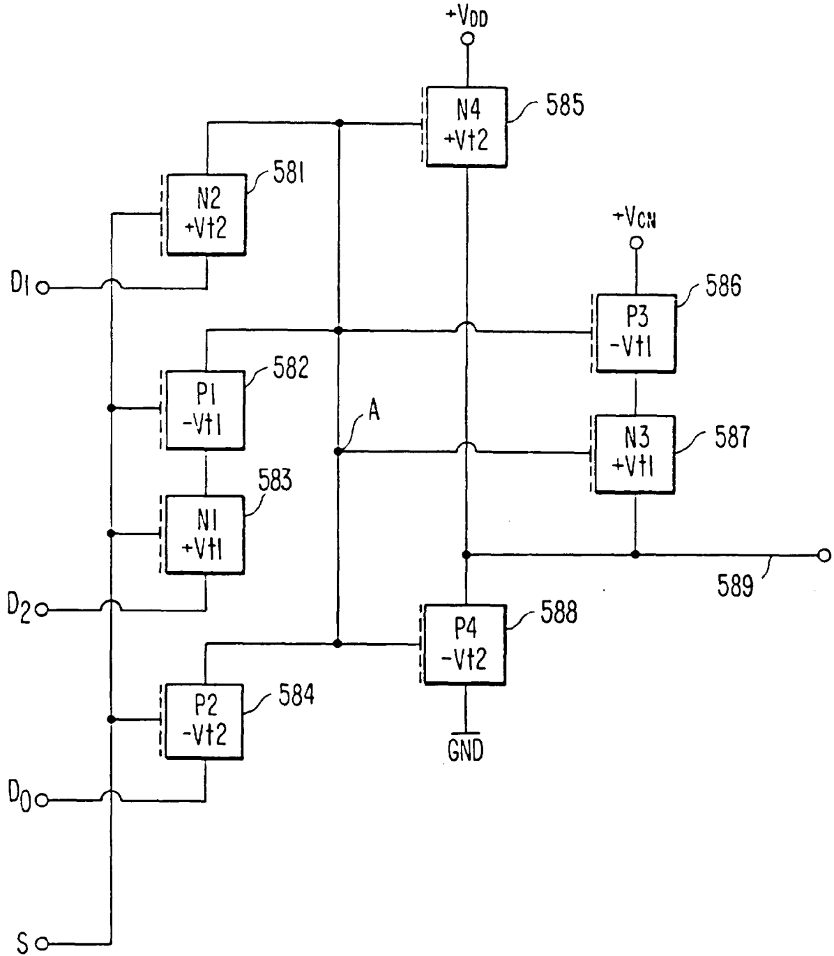
FIG. 16A. TRINARY MULTIPLEXOR
