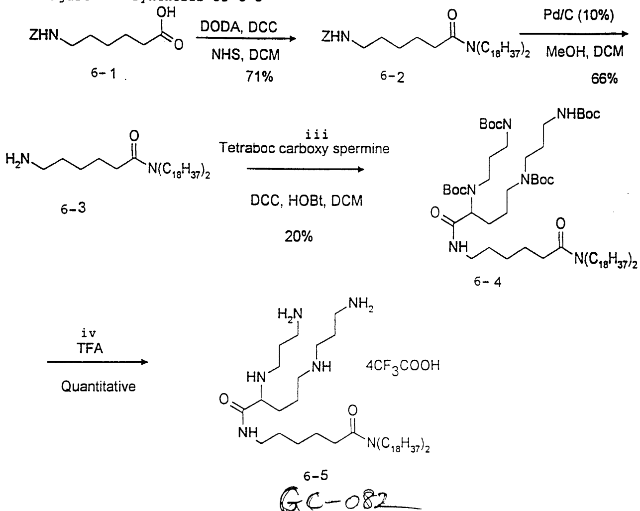
Figure 6: Synthesis of 6-5
