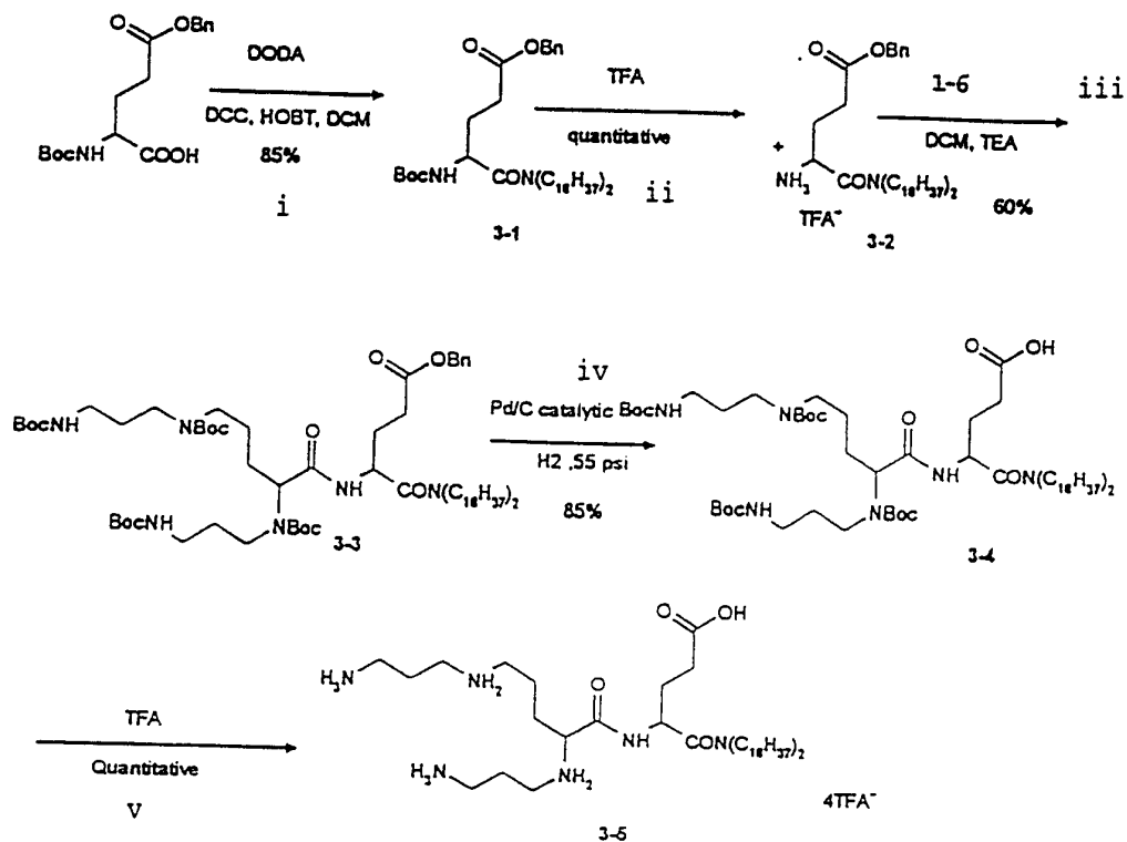
Figure 3: Synthesis of 3-5
