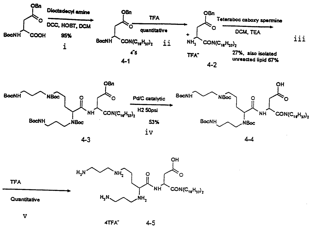
Figure 4 : Synthesis of 4-5
