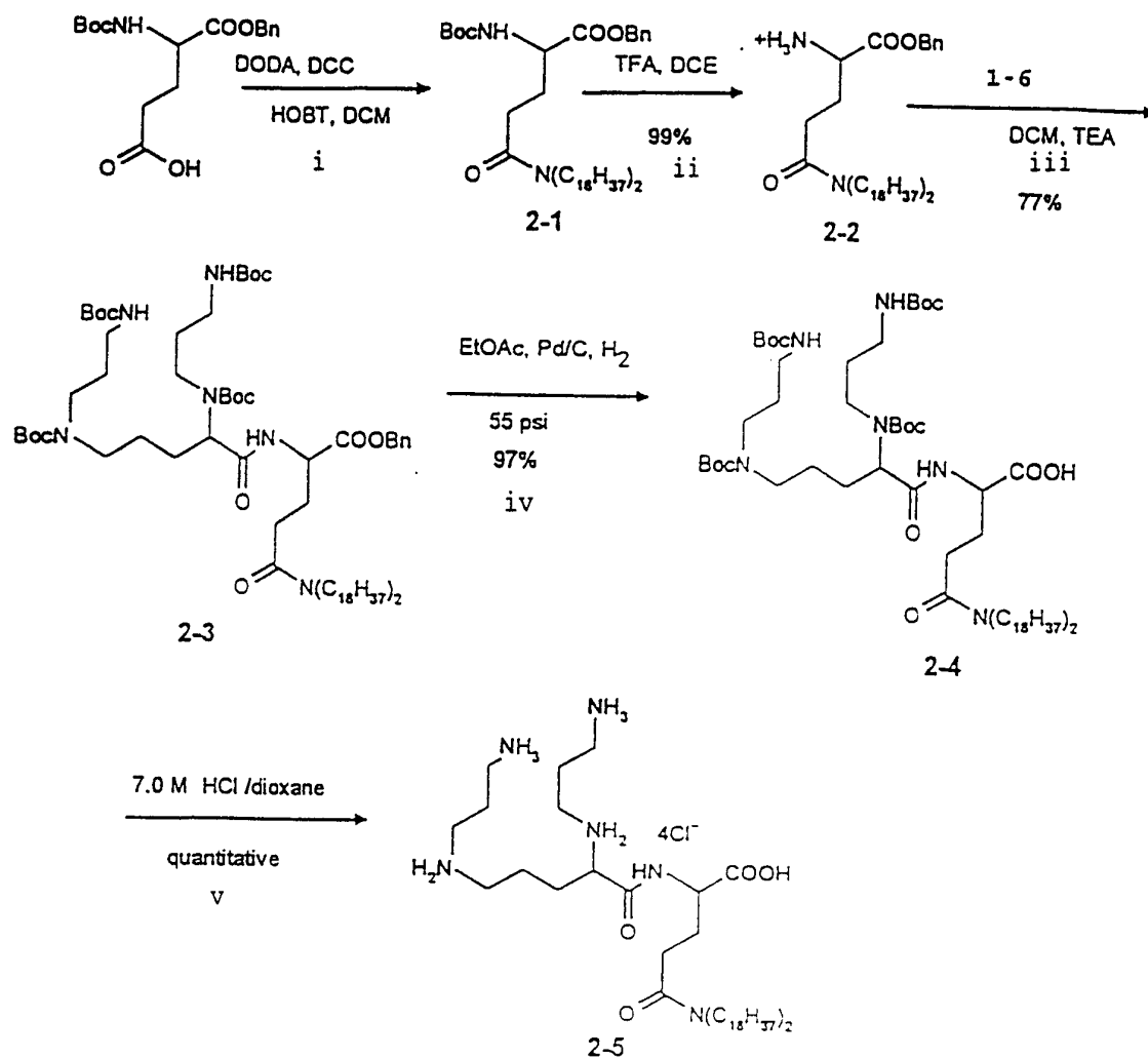
Figure 2: Synthesis of 2-5
