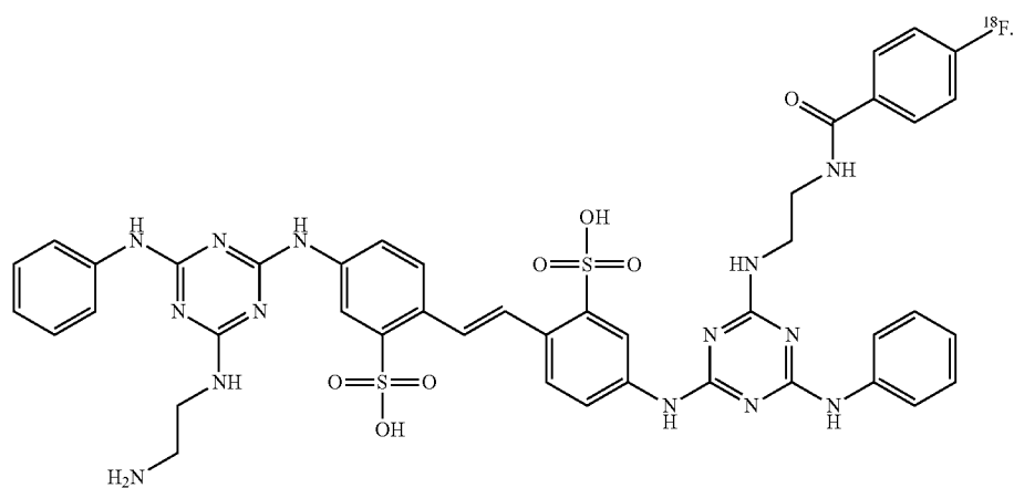
(4-fluorobenzamide)
