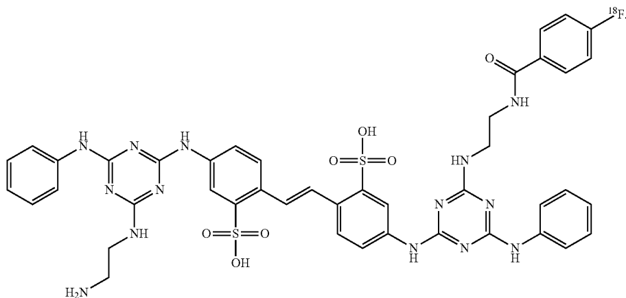
4-fluorobenzamide
