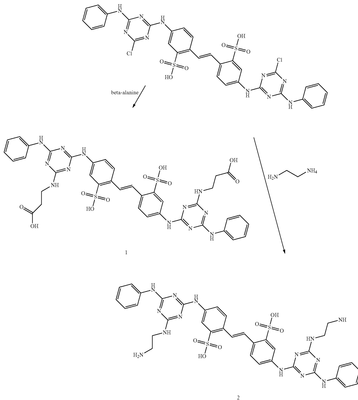
SCHEME 2
