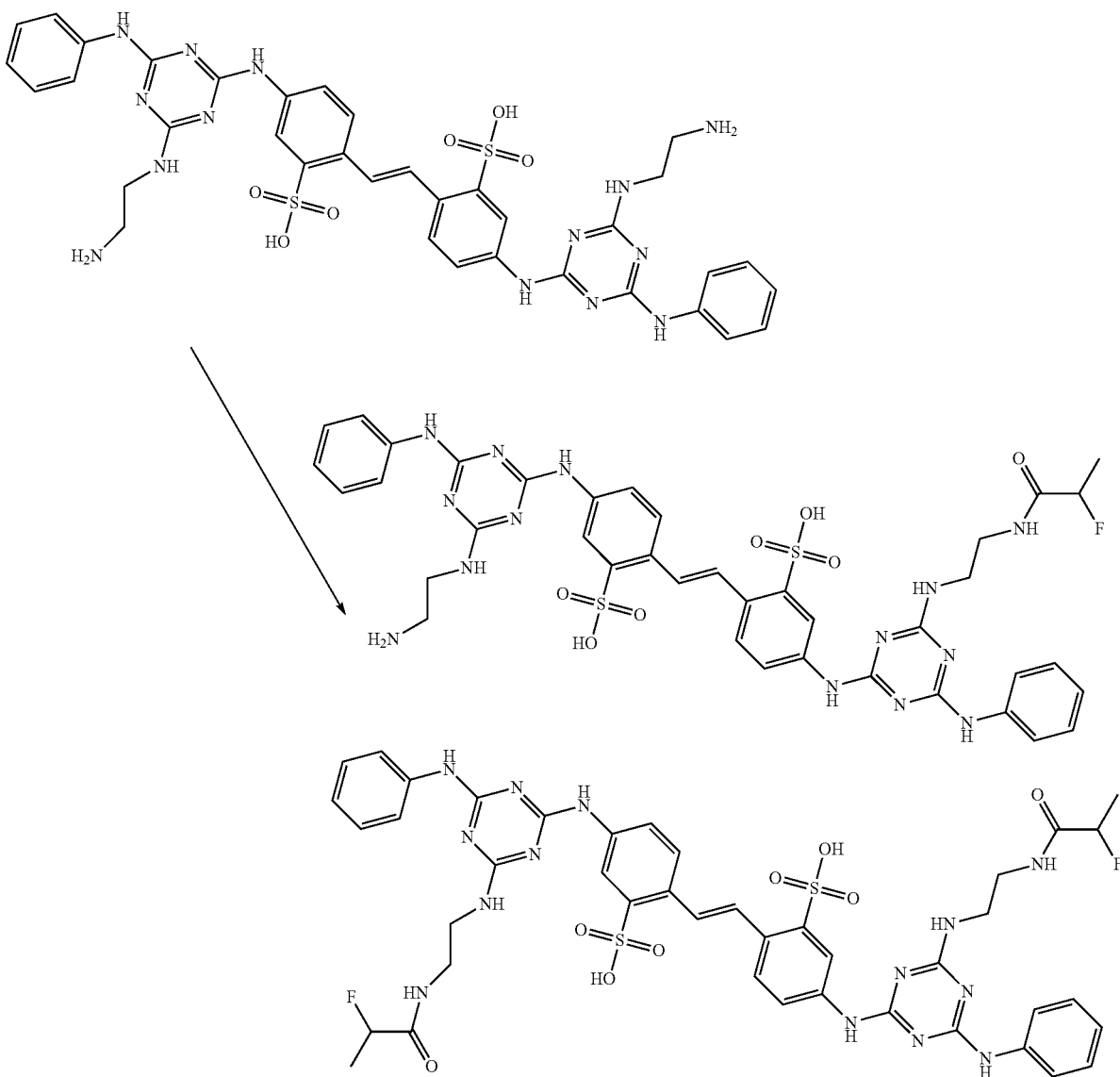
SCHEME 4
