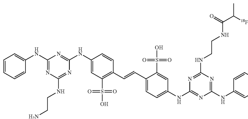
(2-fluoropropanamide)
