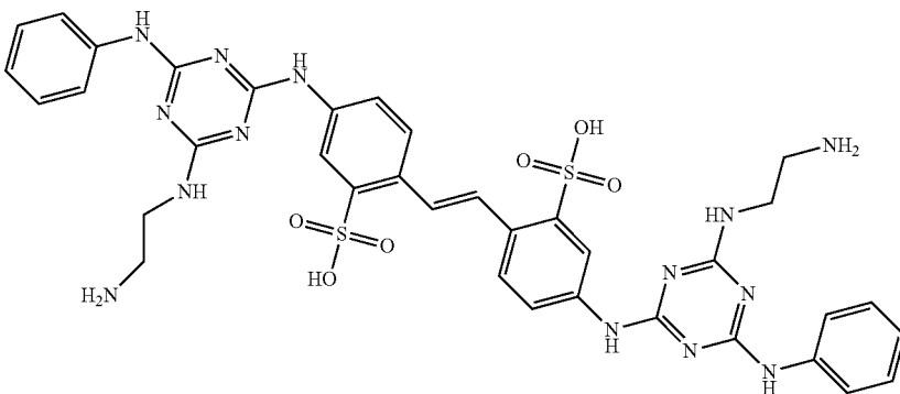
SCHEME 5
