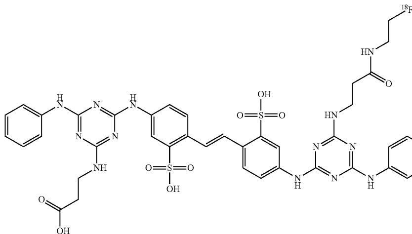
2-fluoroethylamide
