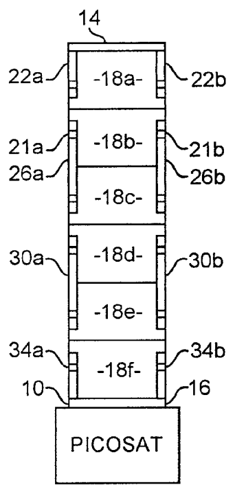
PICO SAT FRONT VIEW FIG. 1B
