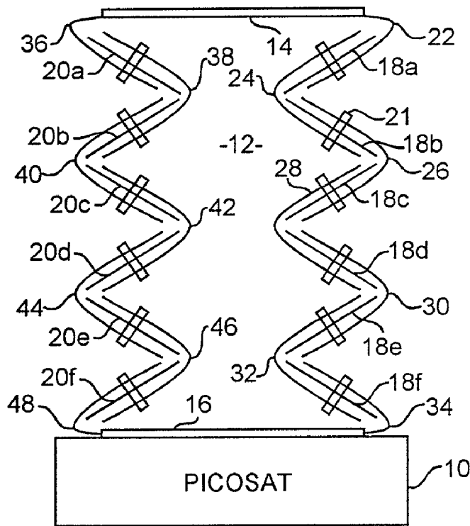
PICOSAT SIDE VIEW
