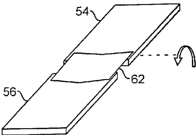
SCALLOPED NITINOL HINGE FIG. 4B
