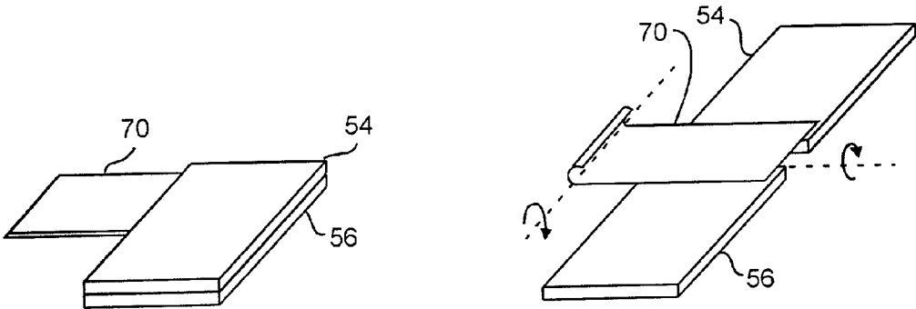
OPENED LATCH FIG. 7B
