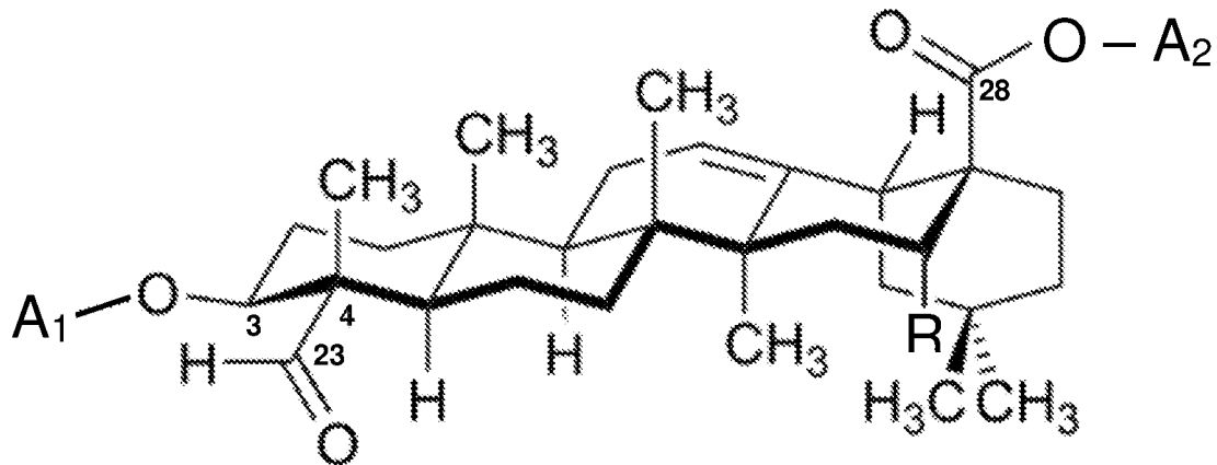
(Molecule 1)
