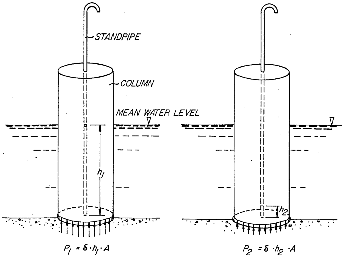
SIMULATED NORMAL OPERATION HOLDDOWN SYSTEM NOT ACTIVATED
