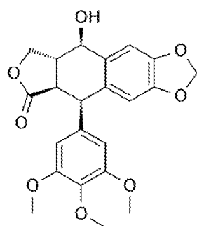
Podophyllotoxin
