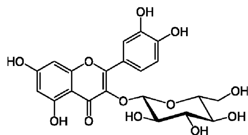
Isoquercetin
