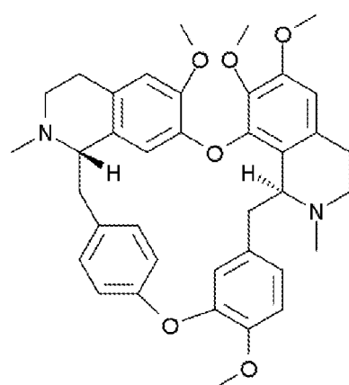
Tetradrine
