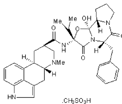
Dihydroergocristine mesylate
