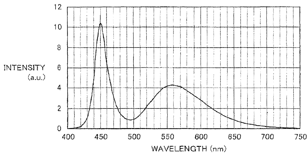
FIG. 7 PRIOR ART
