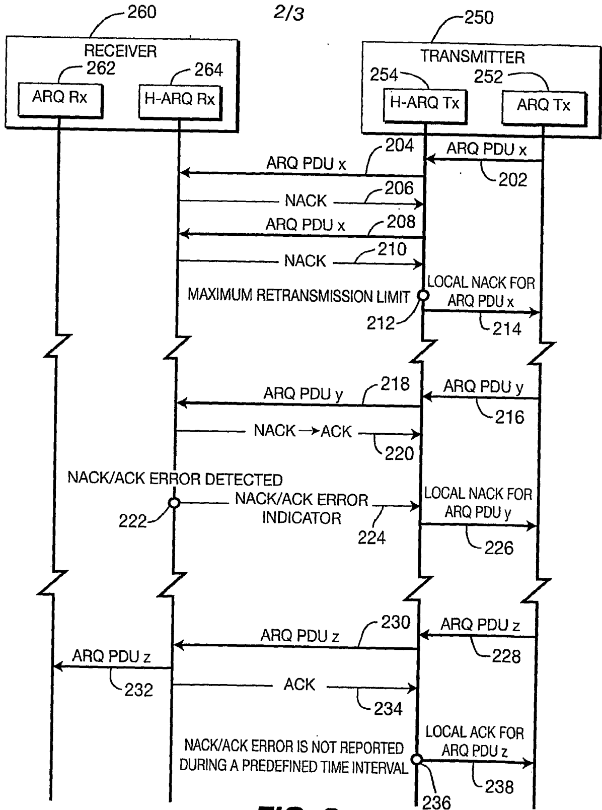
FIG. 2 PRIOR ART
