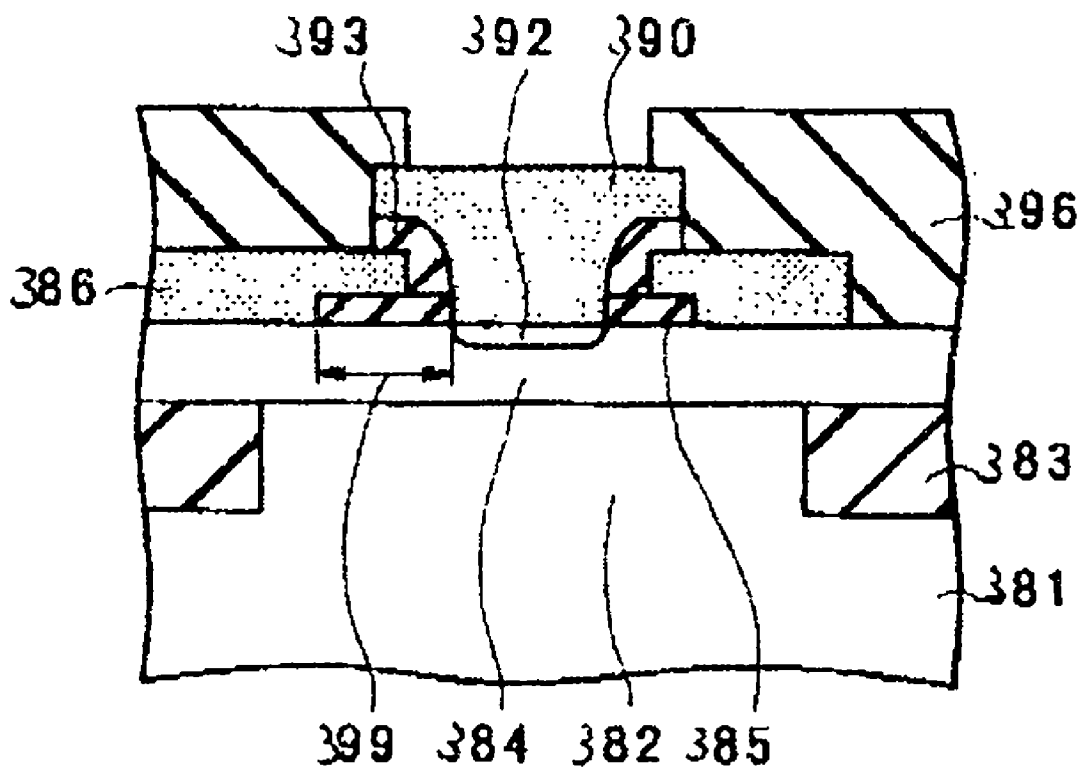
FIG. 15 PRIOR ART
