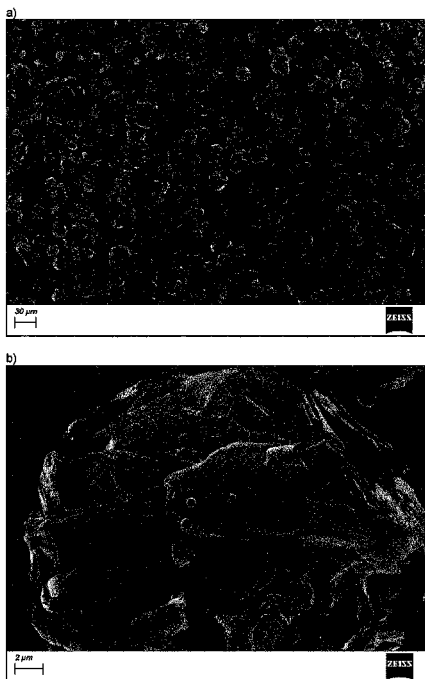
Scanning electron microscopy (SEM) images of carbon intermediate 5 exhibiting non-crystalline binder droplets on the surface
