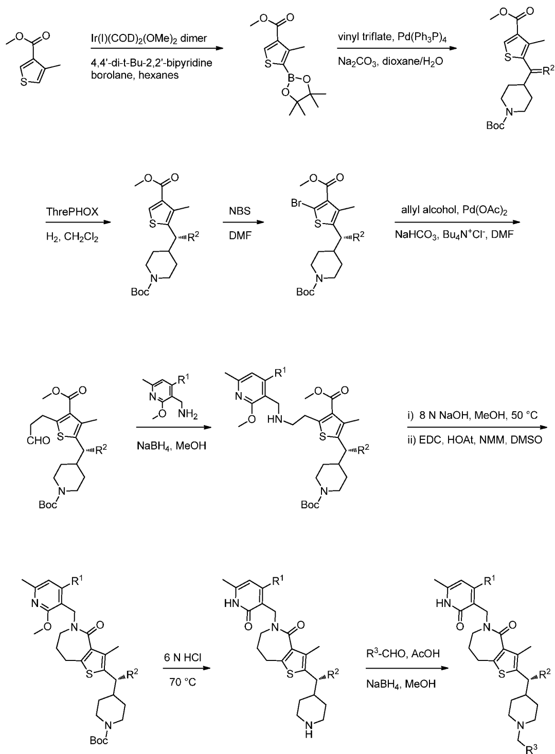
Scheme 1: Synthesis of Compounds of Formula (I).
