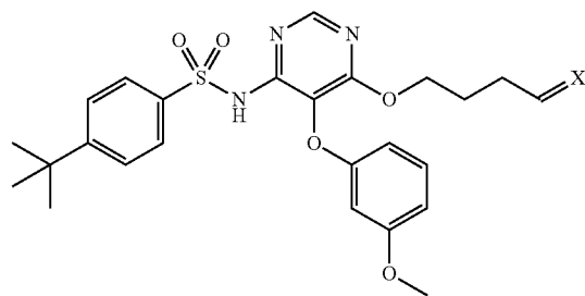
43 X = O 44 X = NNHCO-3-pyridyl
