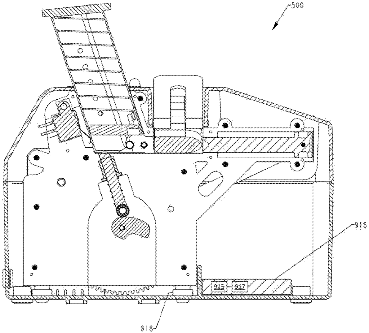
SECTION B-B ROTATED 90° CW FOR CLARITY
