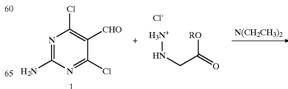
Reaction Scheme 2
