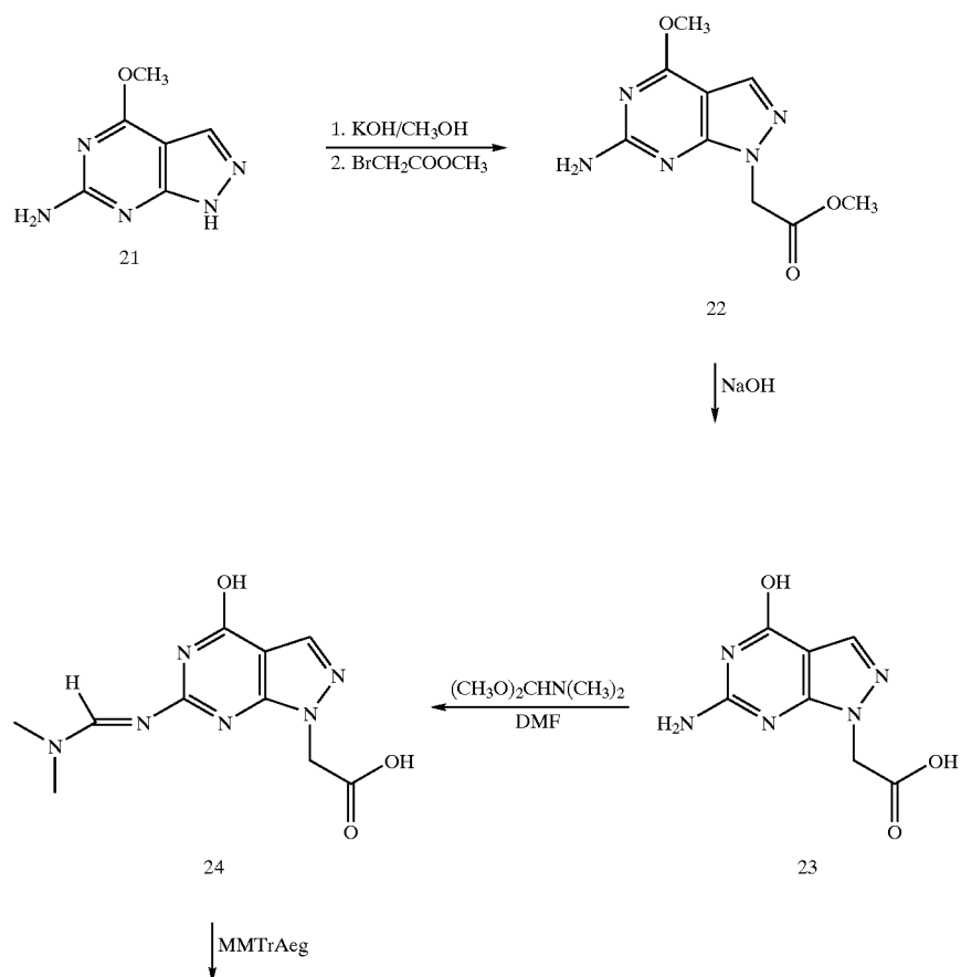
Reaction Scheme 7
