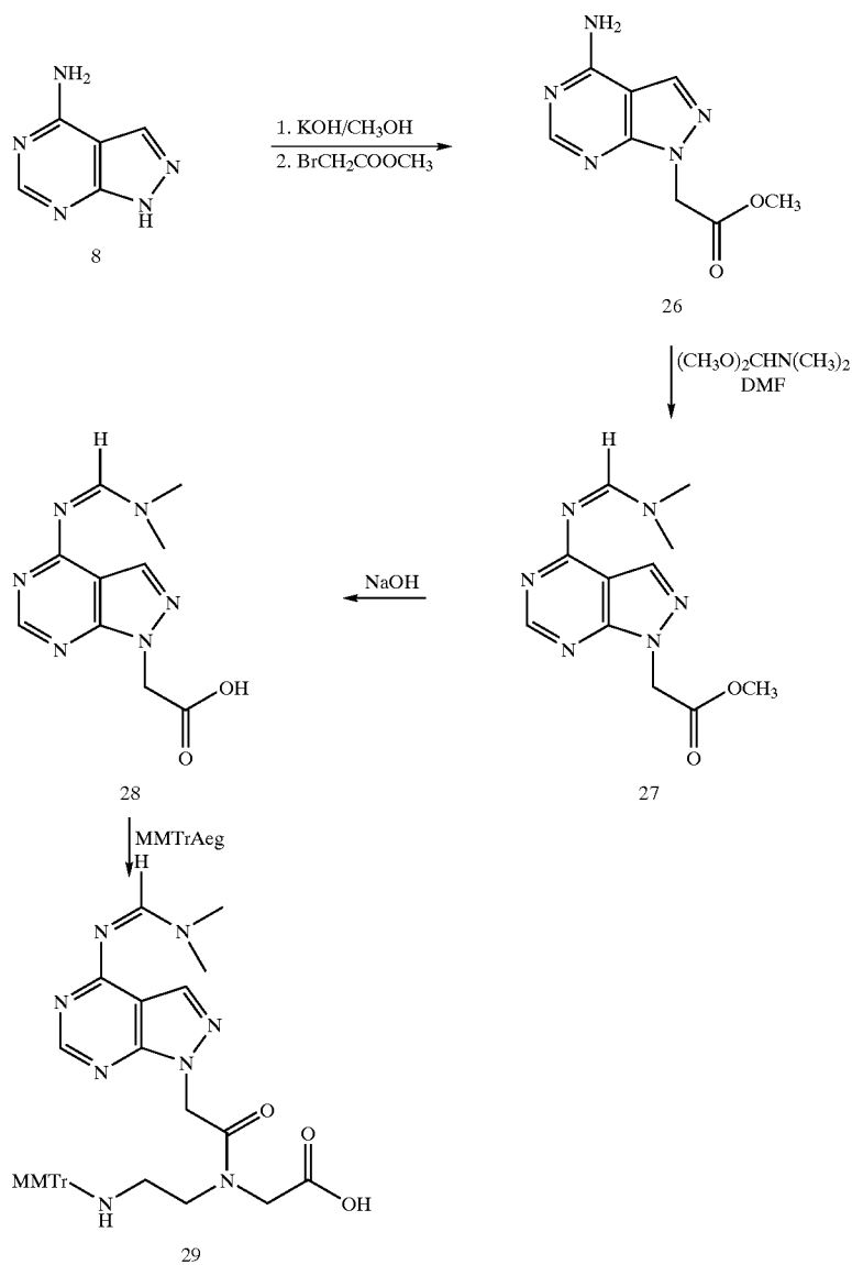
Reaction Scheme 8
