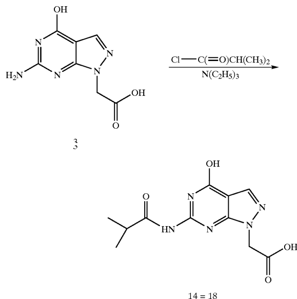
Reaction Scheme 3
