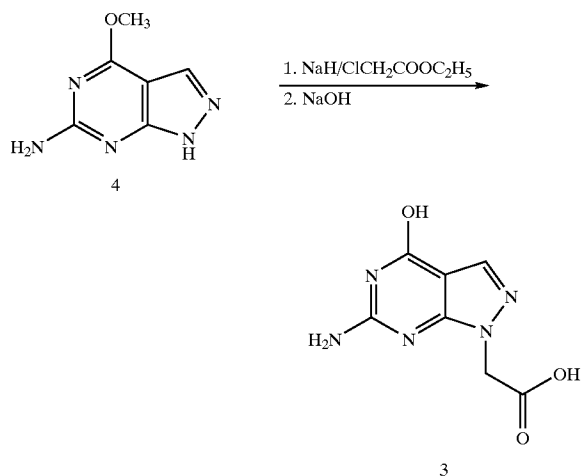
Reaction Scheme 1
