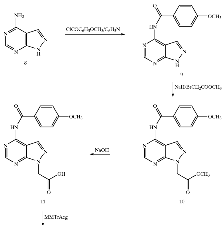
Reaction Scheme 6
