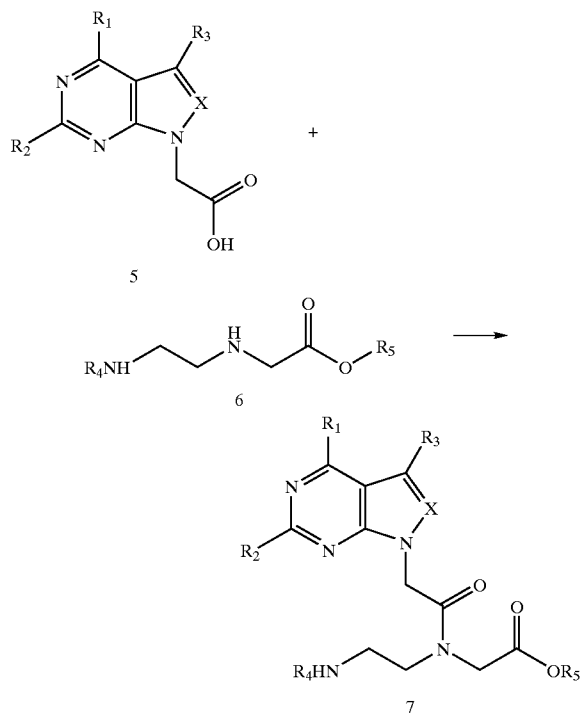
Reaction Scheme 4
