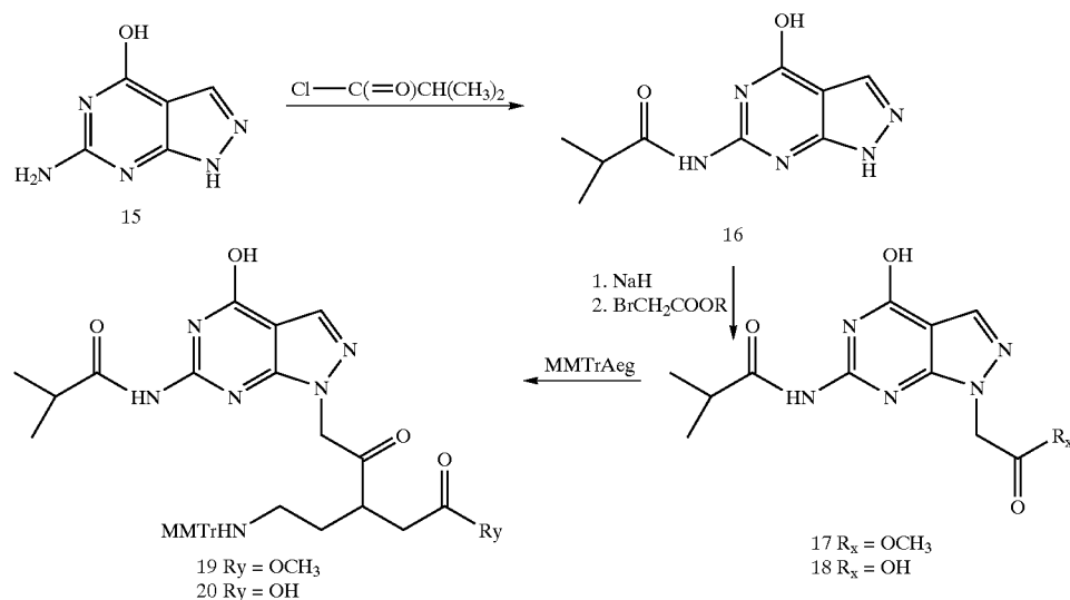
Reaction Scheme 5
