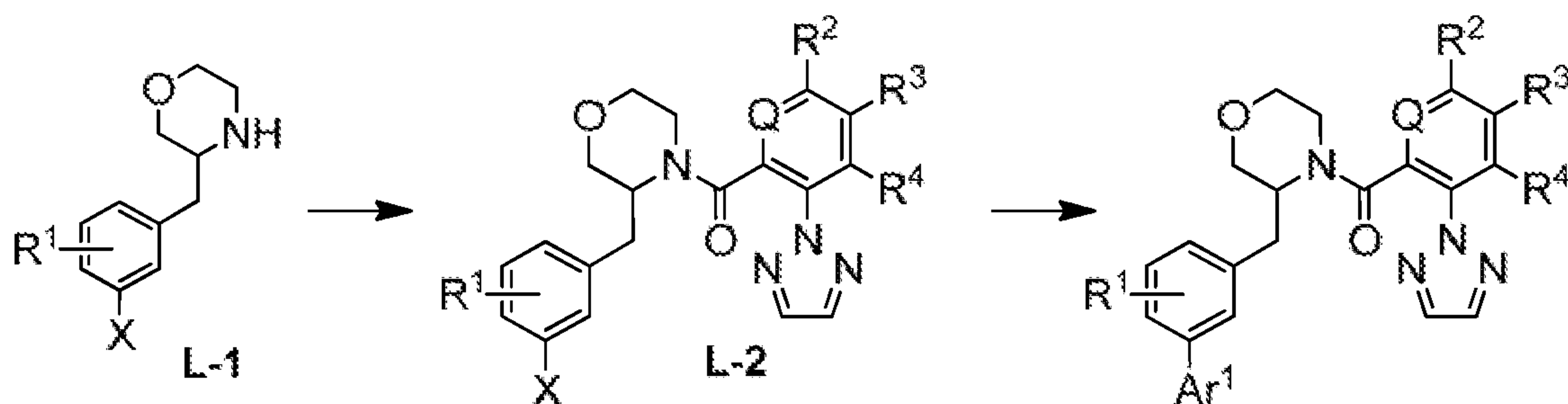
Reaction Scheme L
