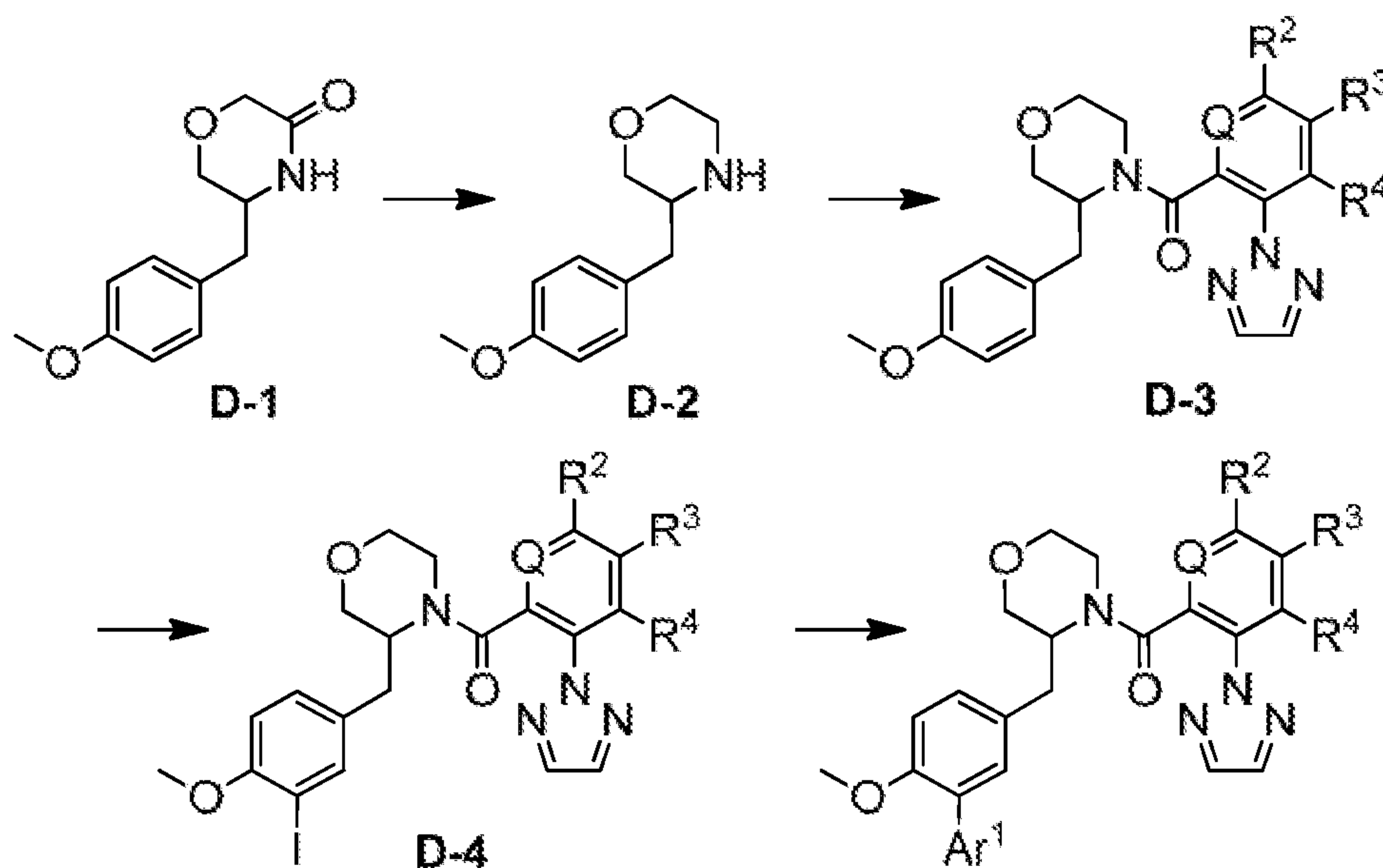
Reaction Scheme D
