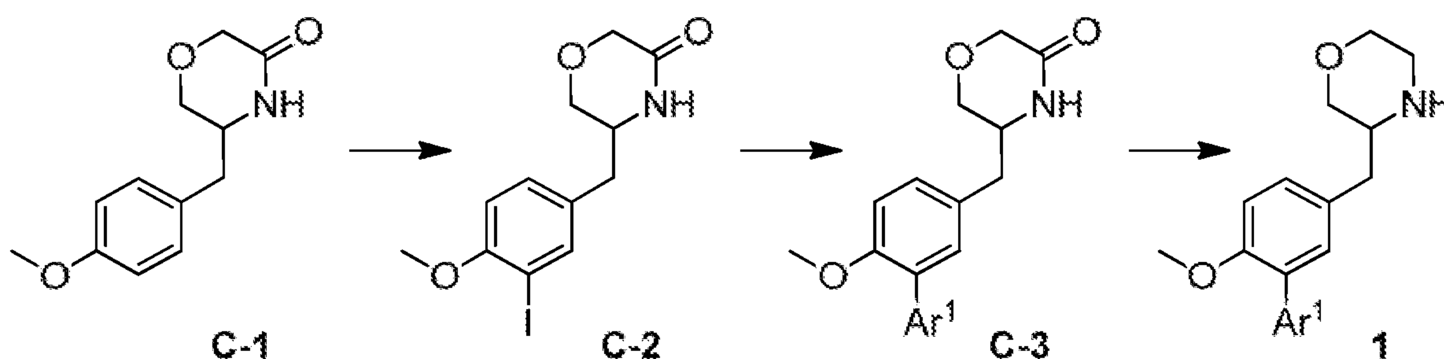
Reaction Scheme C
