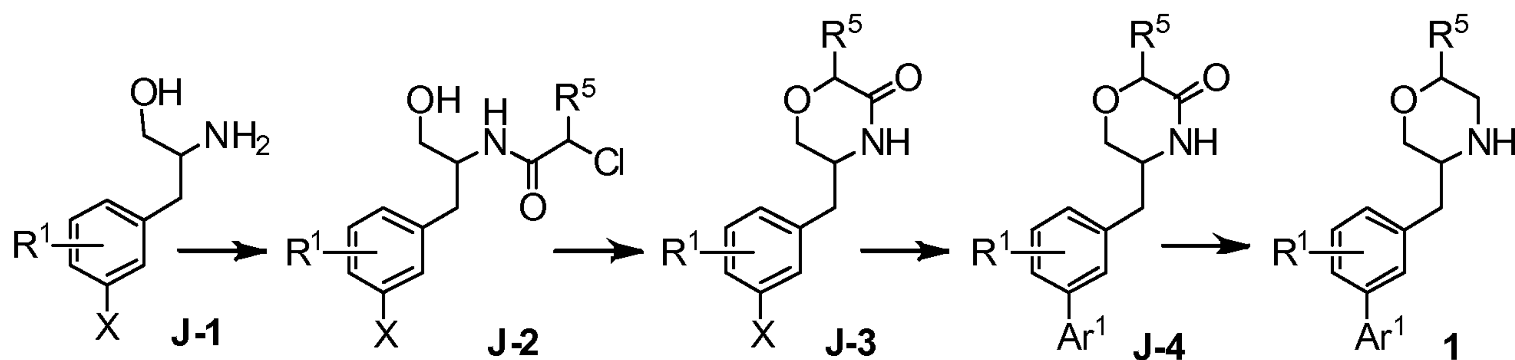
Reaction Scheme J
