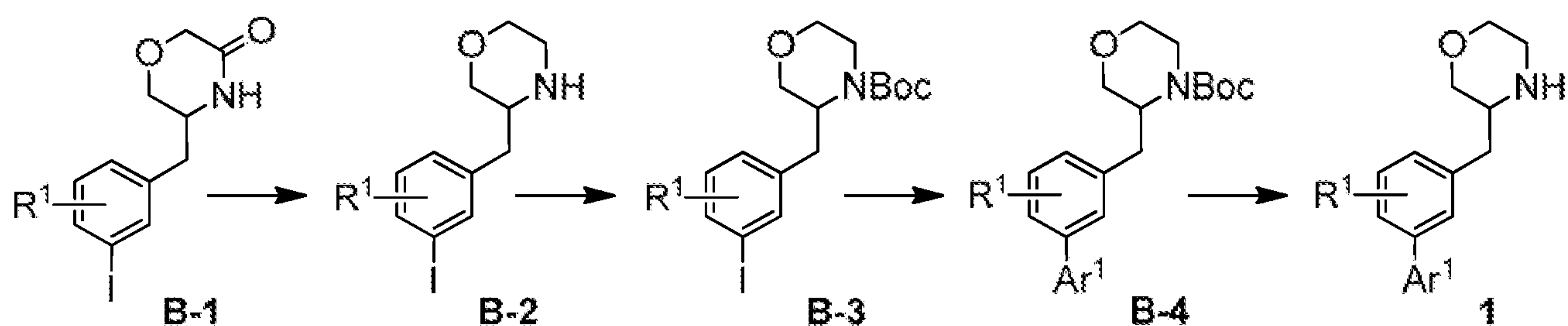
Reaction Scheme B
