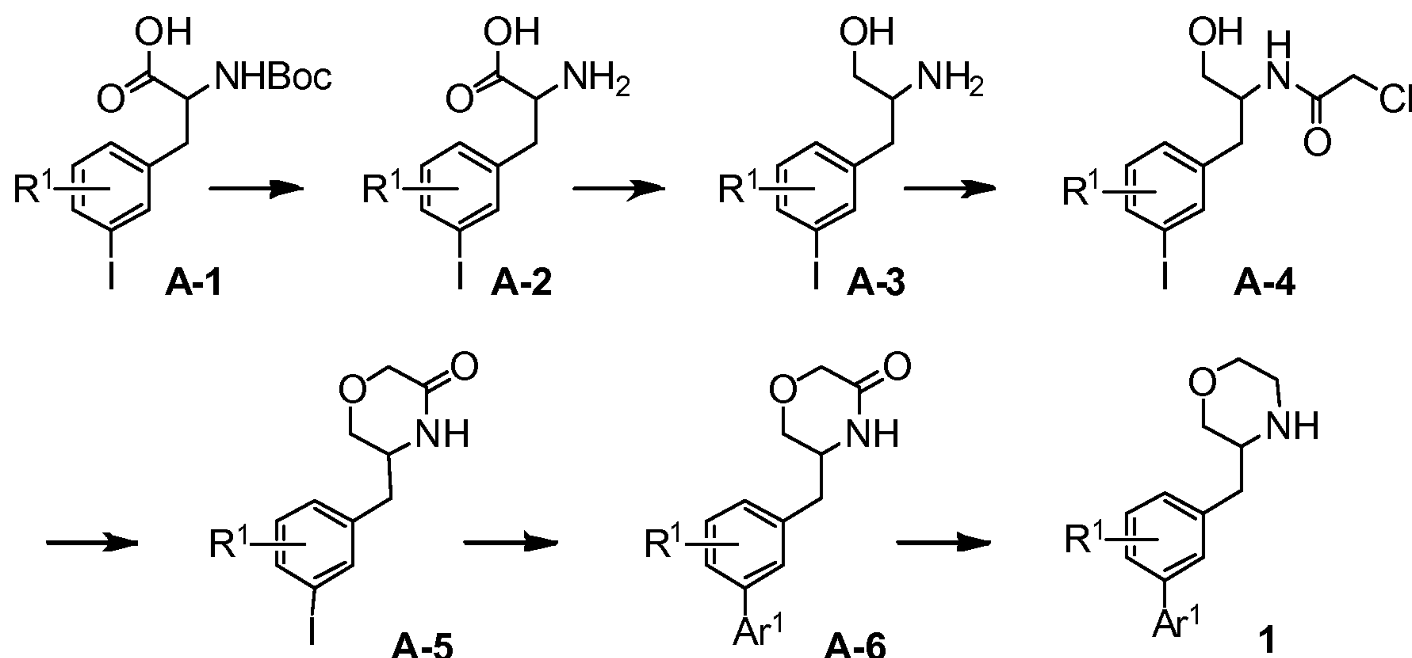
Reaction Scheme A
