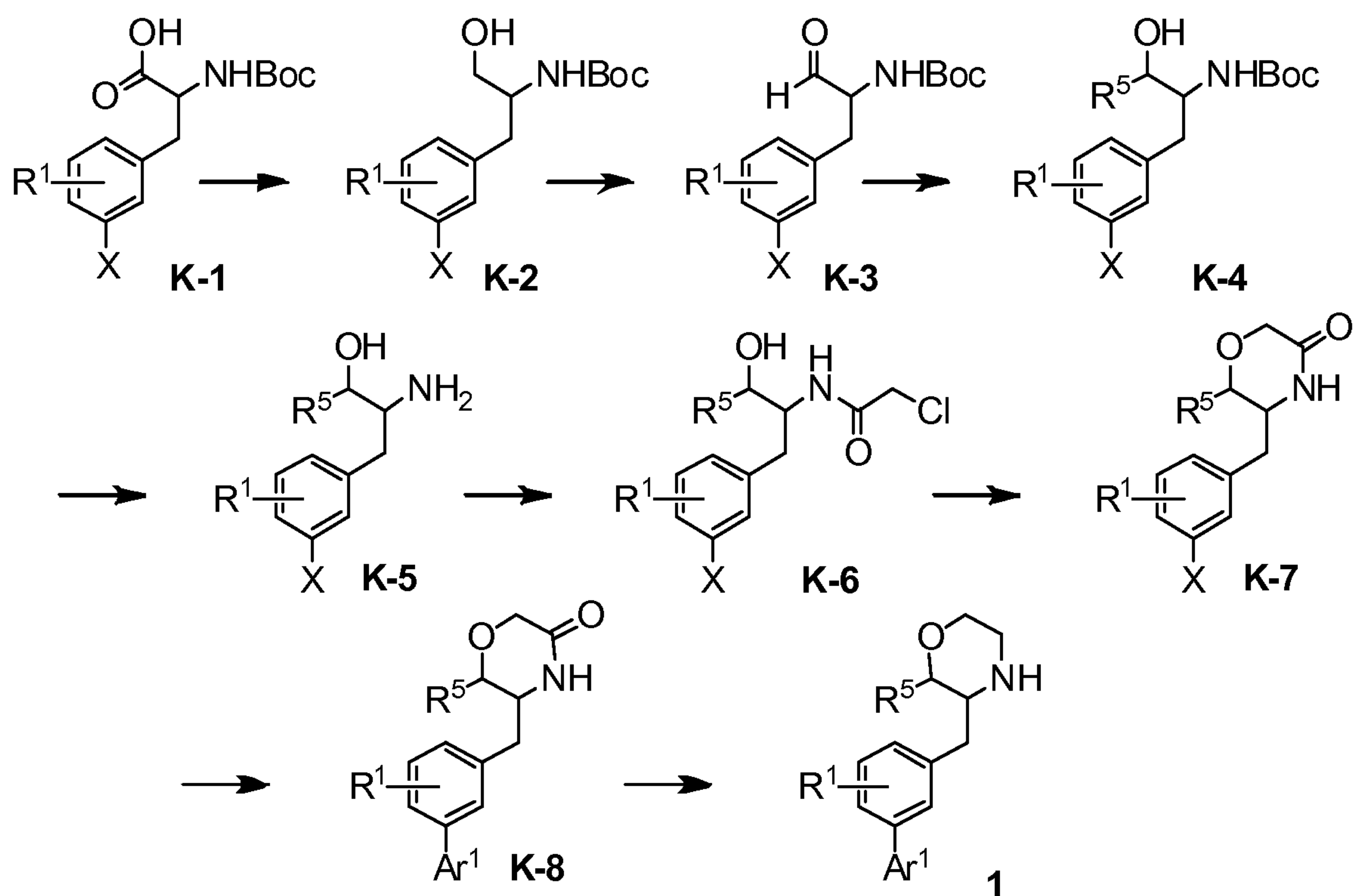
Reaction Scheme K
