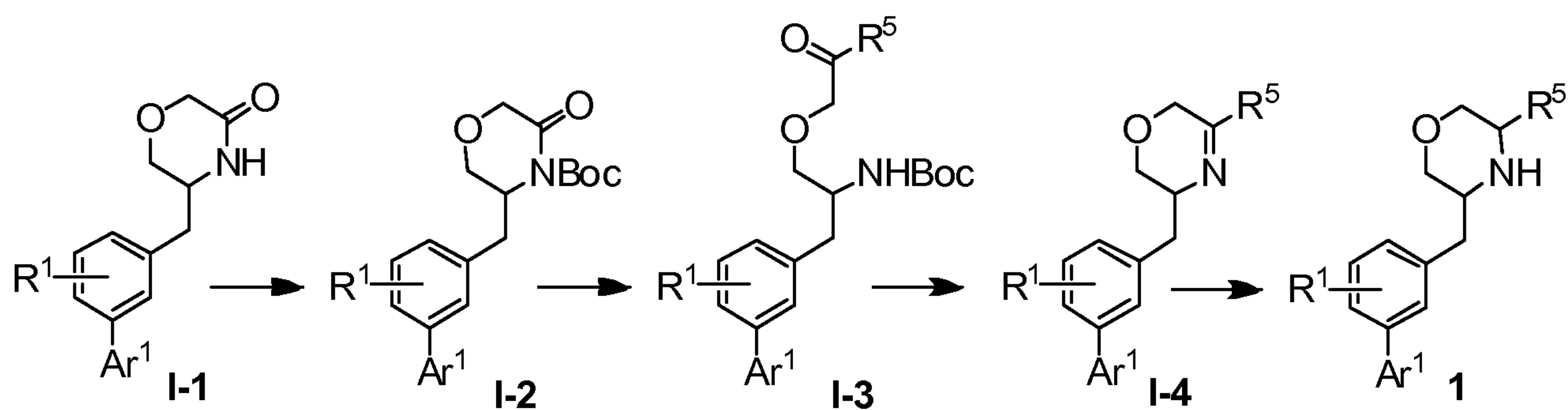
Reaction Scheme I
