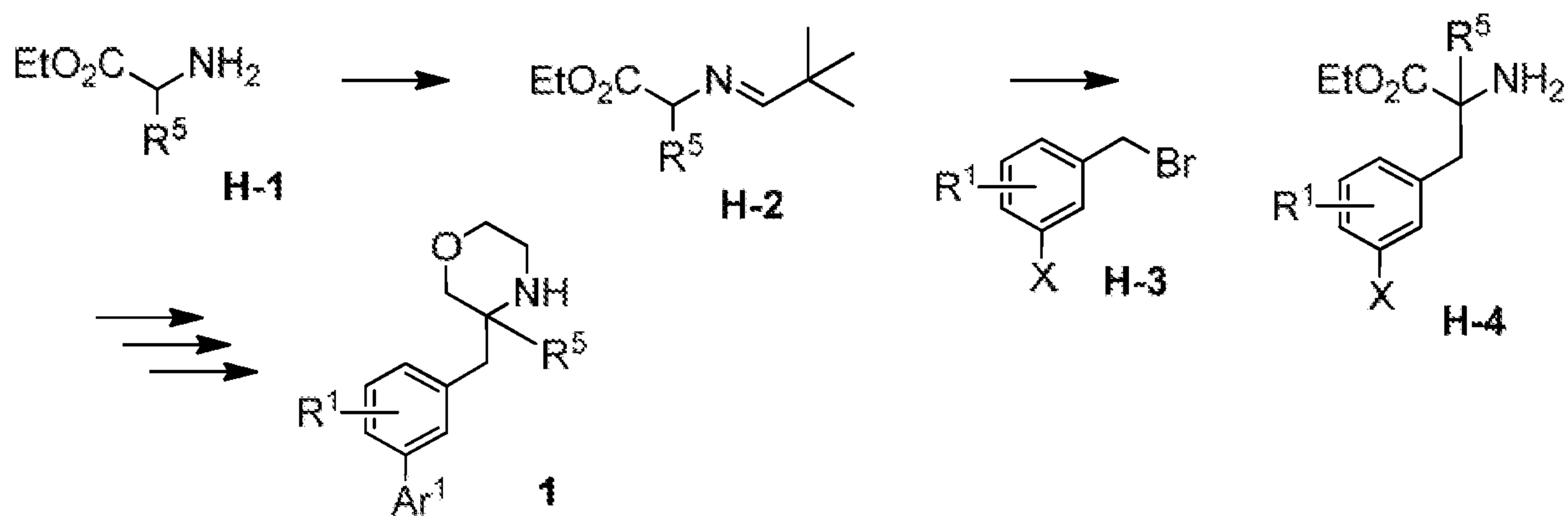
Reaction Scheme H
