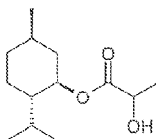
l-menthyl lactate
