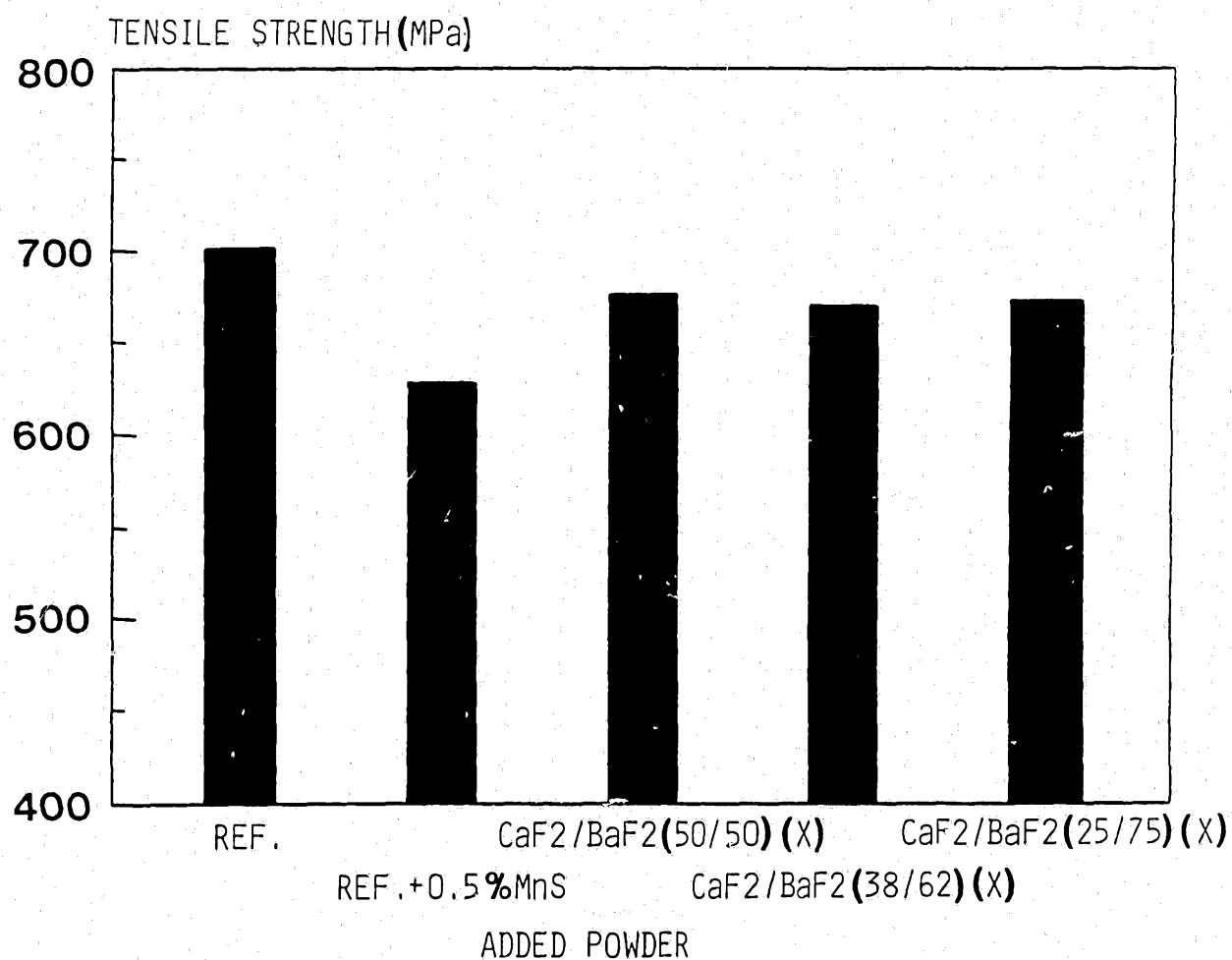
FIG. 2b: TENSILE STRENGTH OF Fe-4%Ni-1.5%Cu-0.5%Mo-0.5%C WITH ADDITION OF 0.6%CaF 2 /BaF 2 (VARYING WEIGHT RATIO) +0.2%MnS
