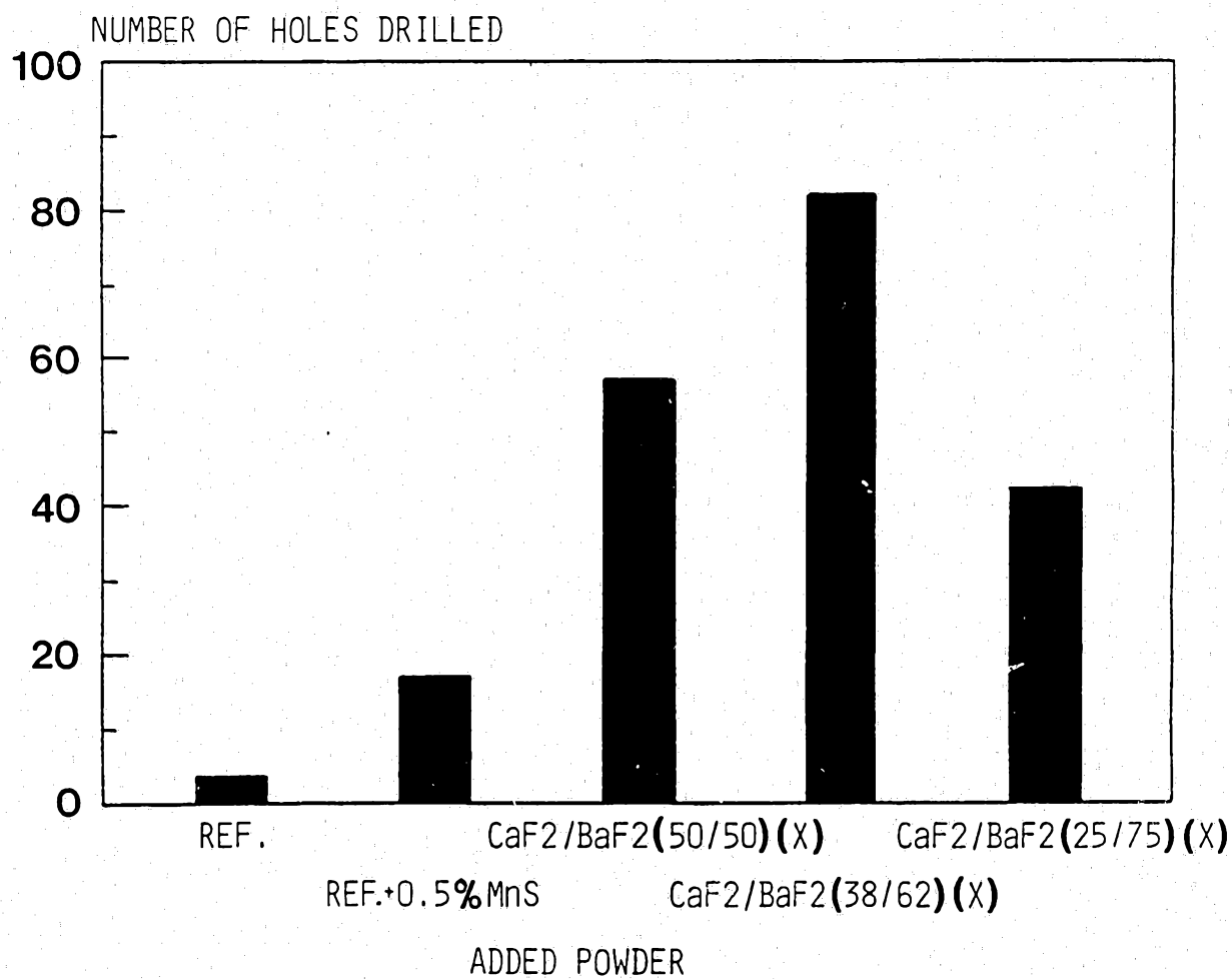
FIG.2a: MACHINABILITY OF Fe-4%Ni-1.5%Cu-0.5%Mo-0.5%C WITH ADDITION OF 0.6%CaF 2 /BaF 2 (VARYING WEIGHT RATIO)+0.2%MnS
