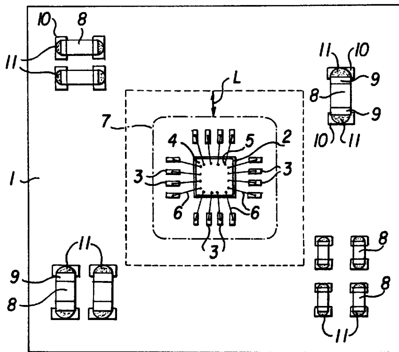
FIG. 12 (PRIOR ART)
